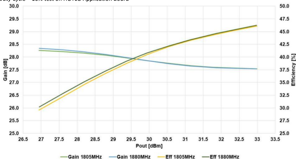
WCDMA, Gain and Efficiency vs Pout
