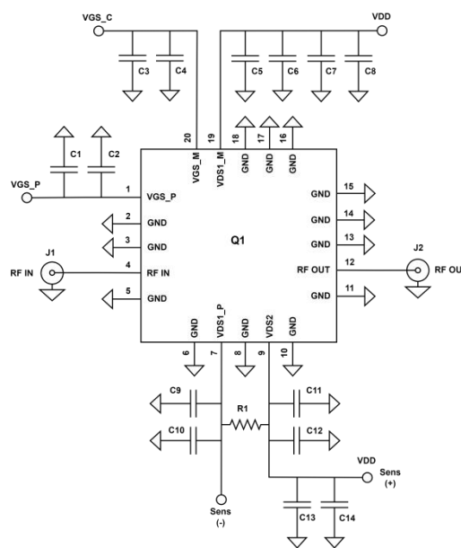
EVb Schematic
