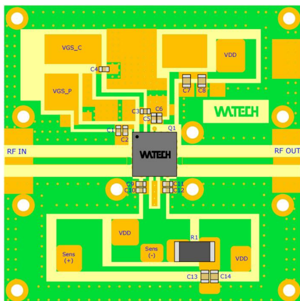
EVb Layout
