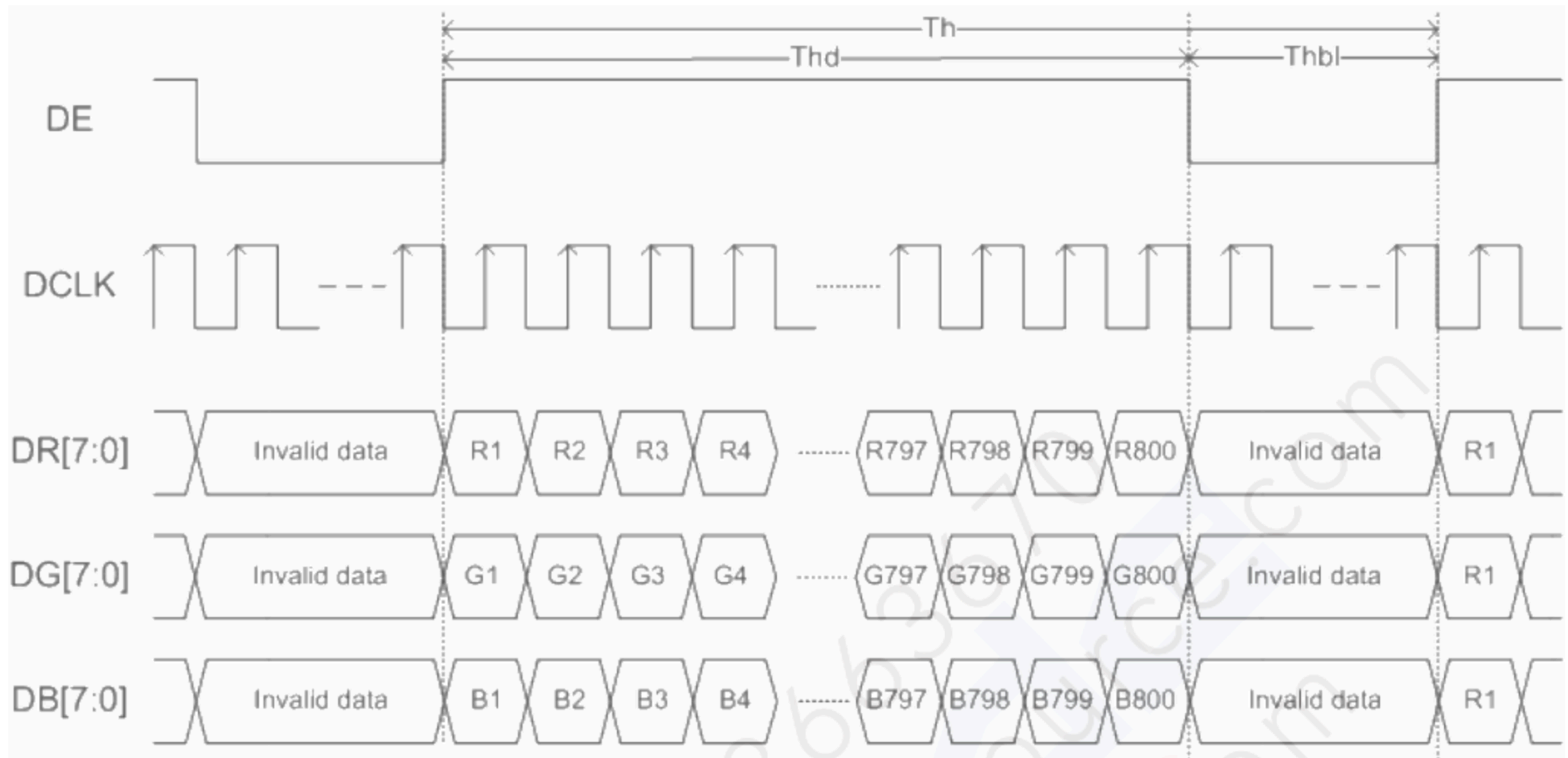
Horizontal input timing
