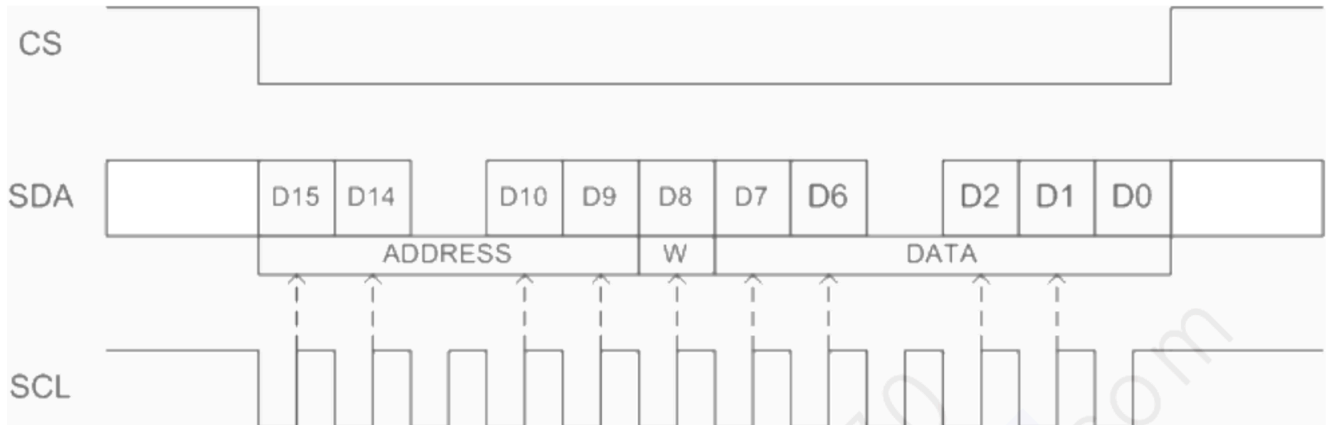
Figure. Serial interface read sequence
