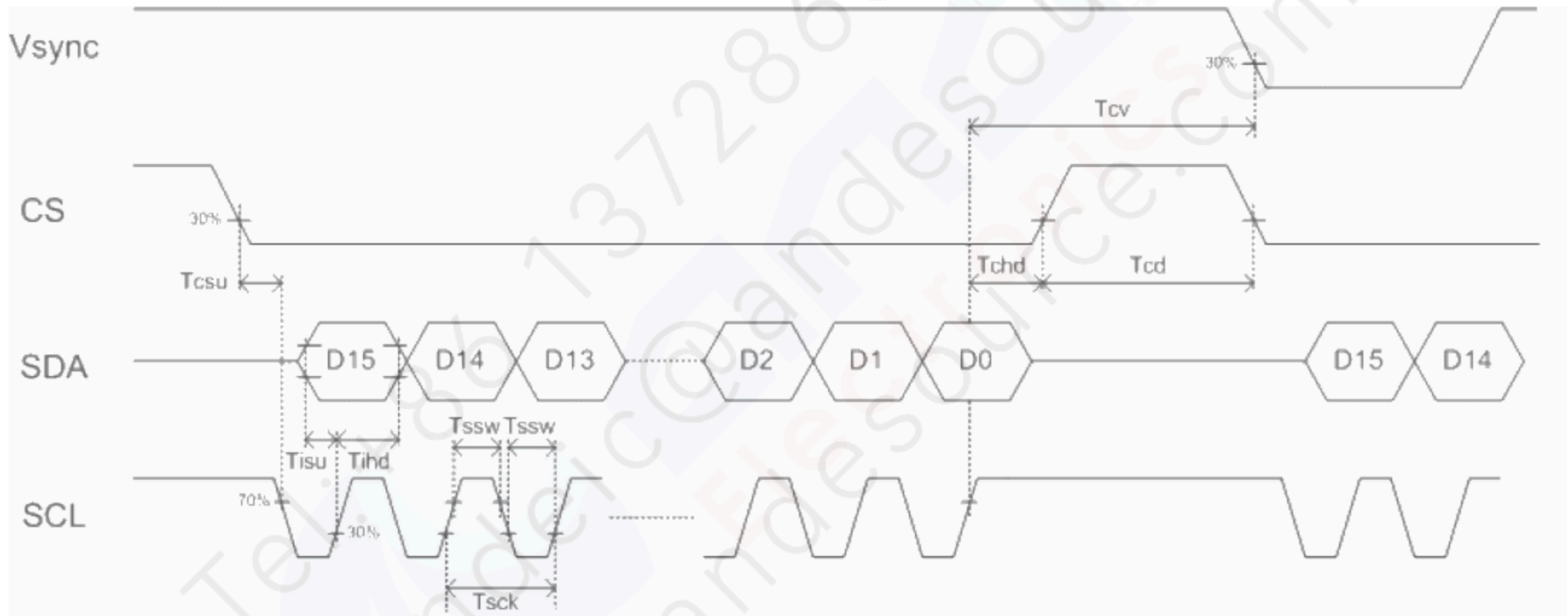
AC serial interface write mode timings
