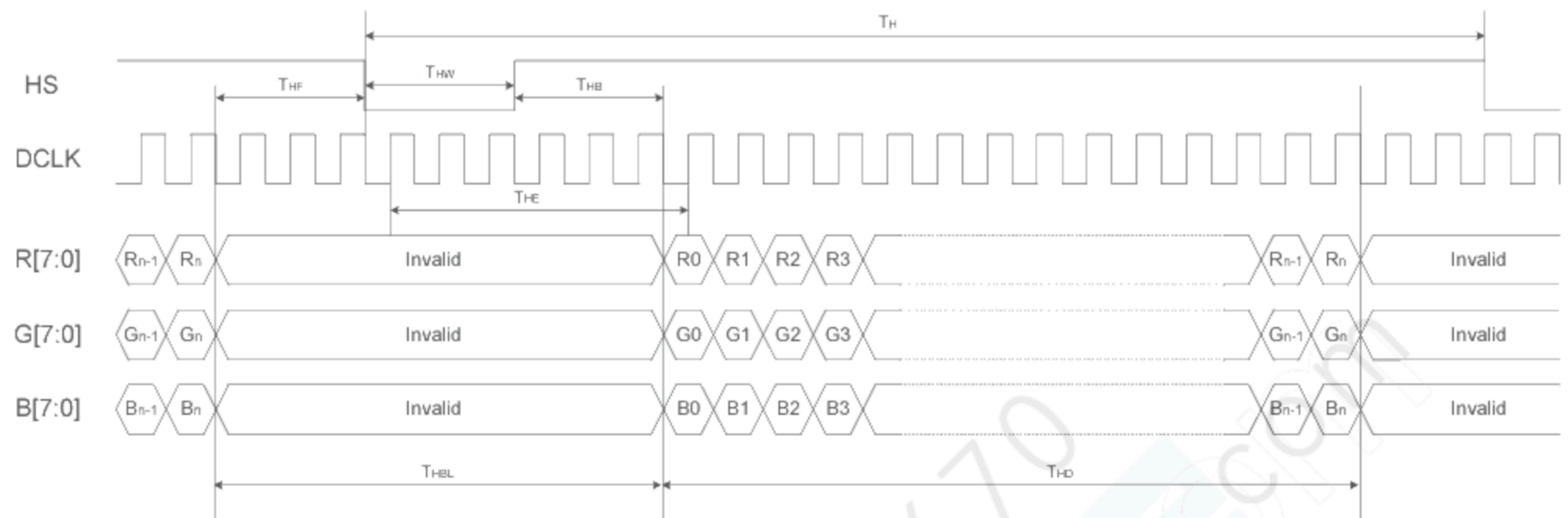
Horizontal input timing. (HV mode)
