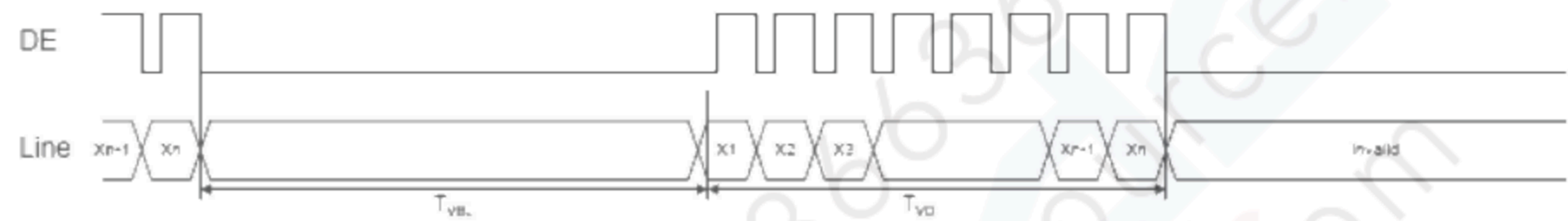
Vertical timing (DE mode)
