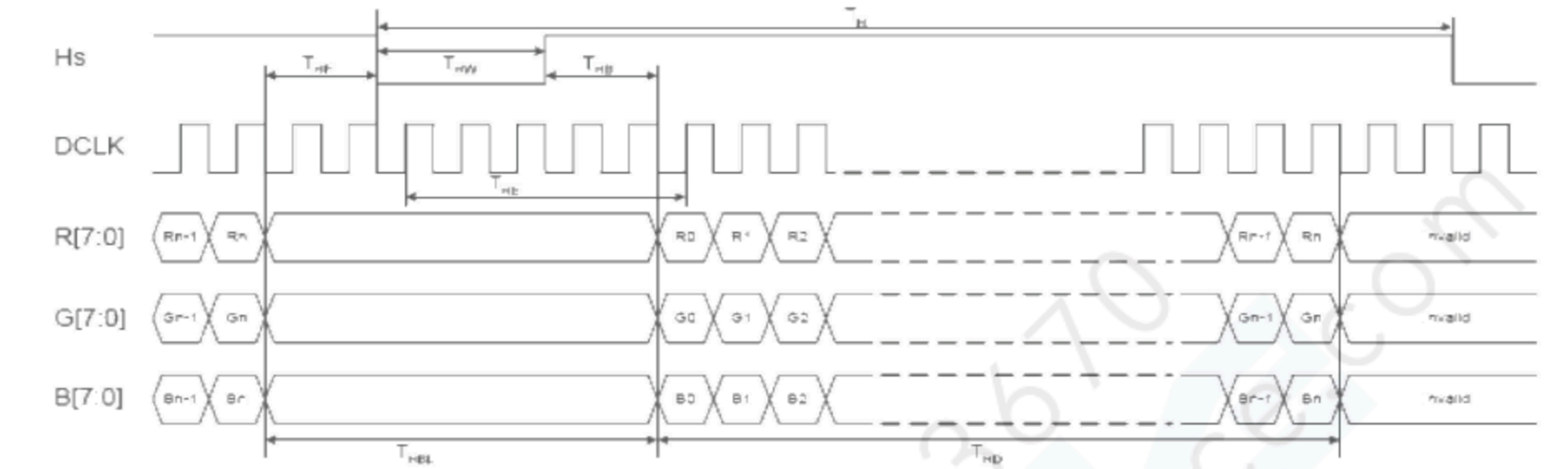
Horizontal input timing (HV mode)
