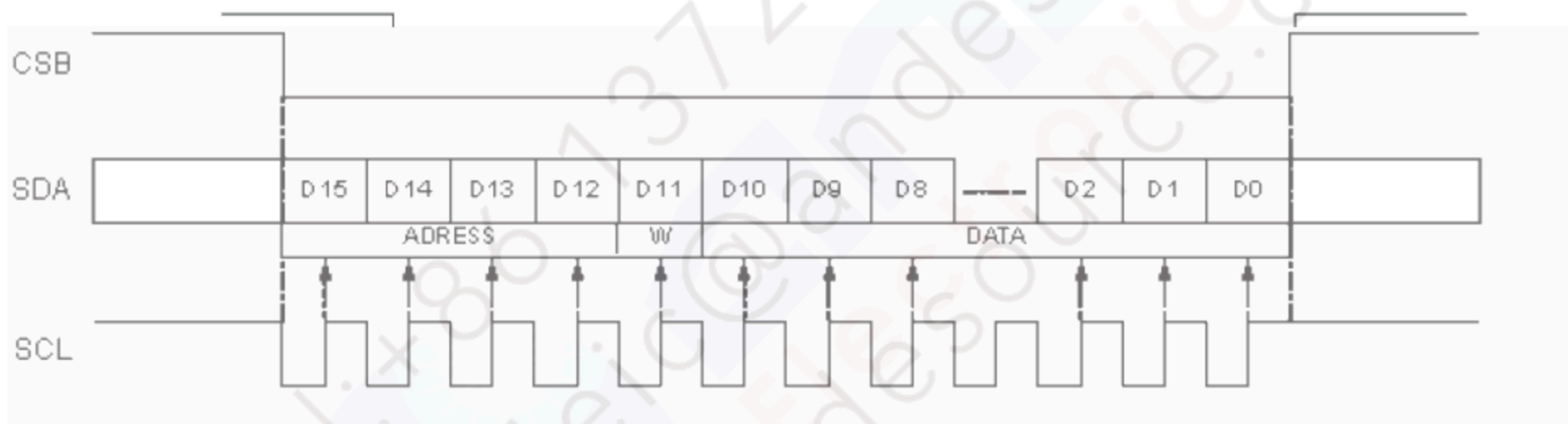
Serial Interface Write sequence
