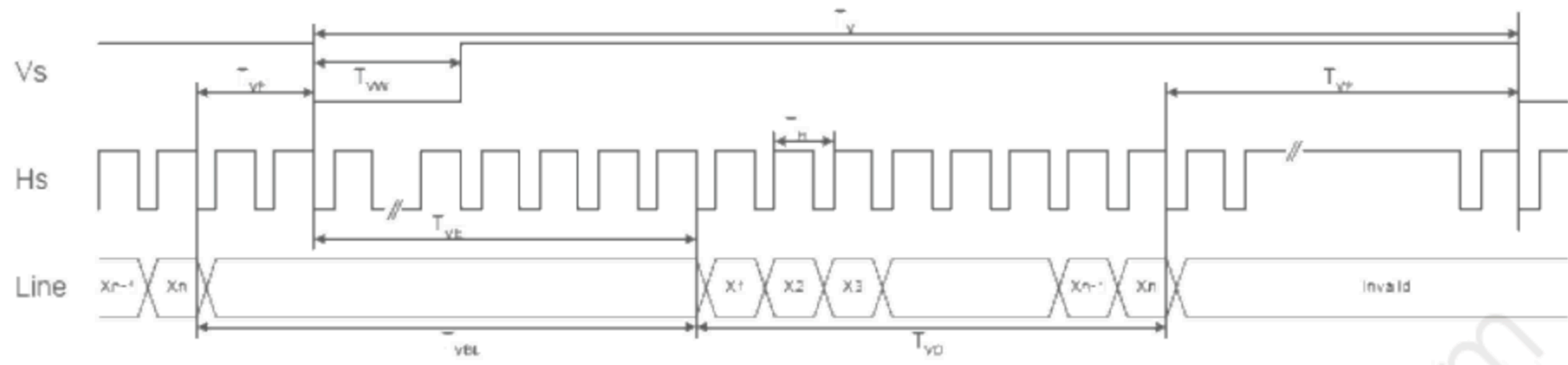
Vertical timing (HV mode)
