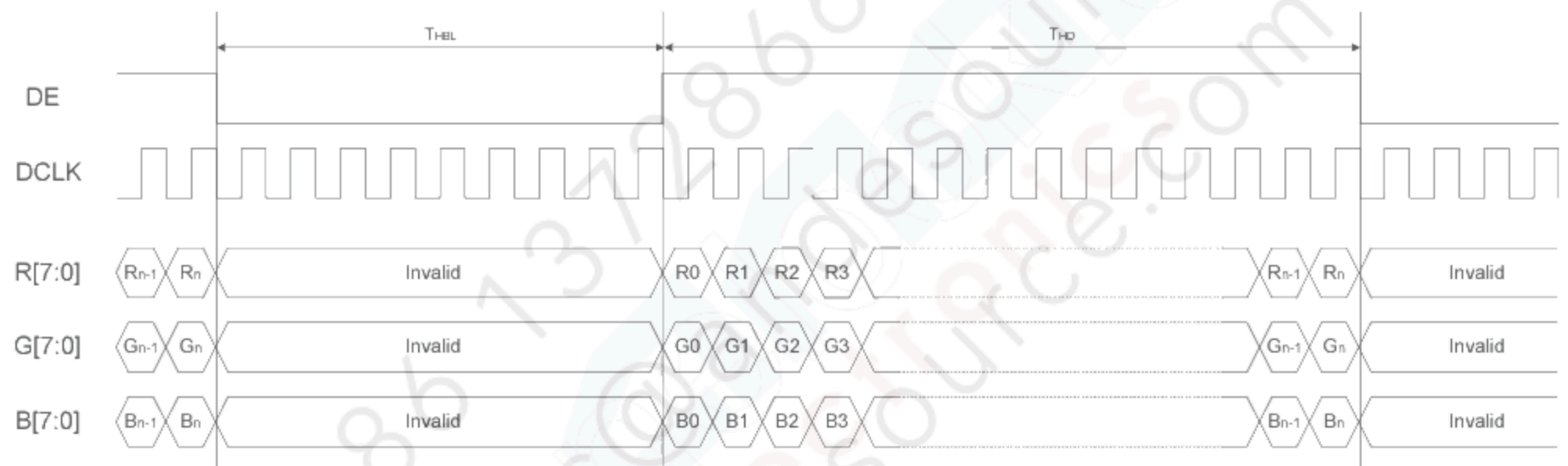
Horizontal input timing. (DE mode)
