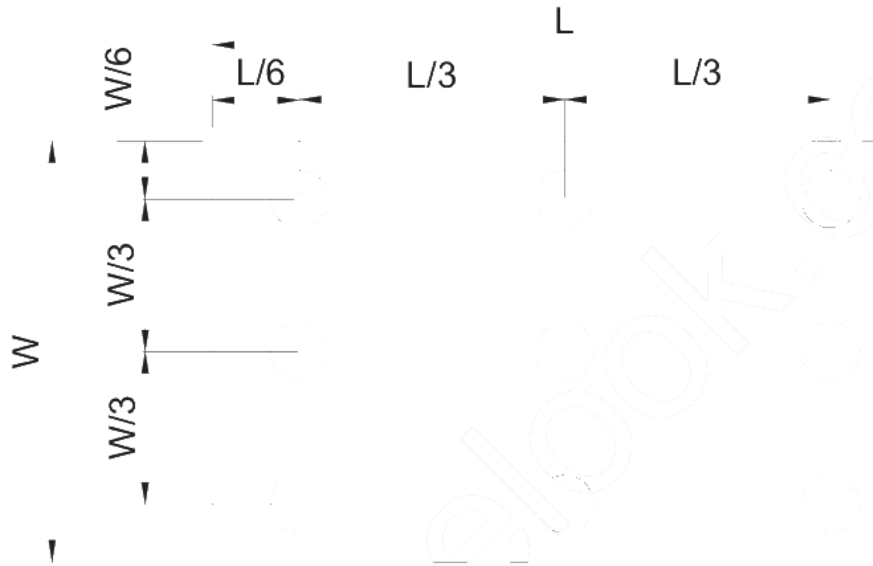
Fig. 4-4 Definition of measuring points
