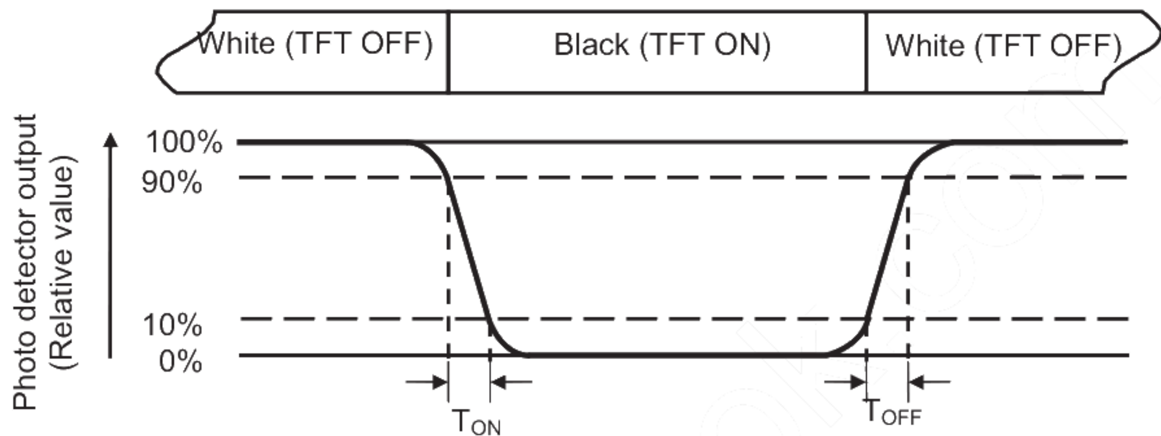
Fig. 4-3 Definition of response time
