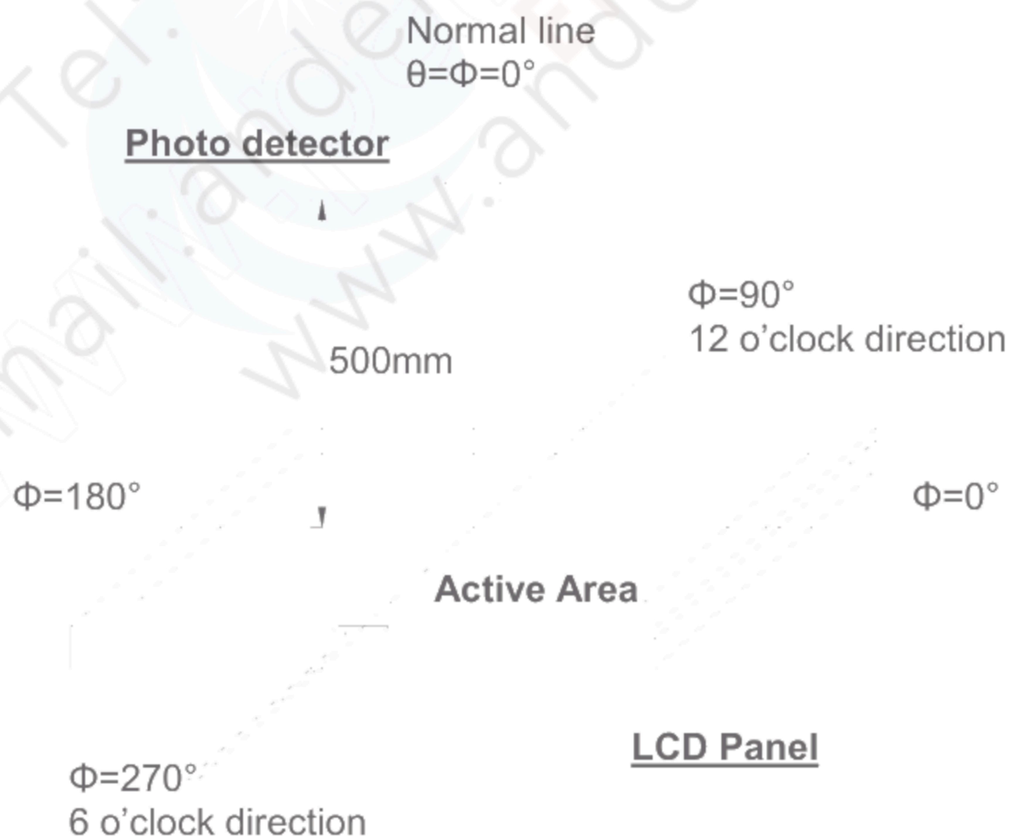
Fig. 4-2 Optical measurement system setup
