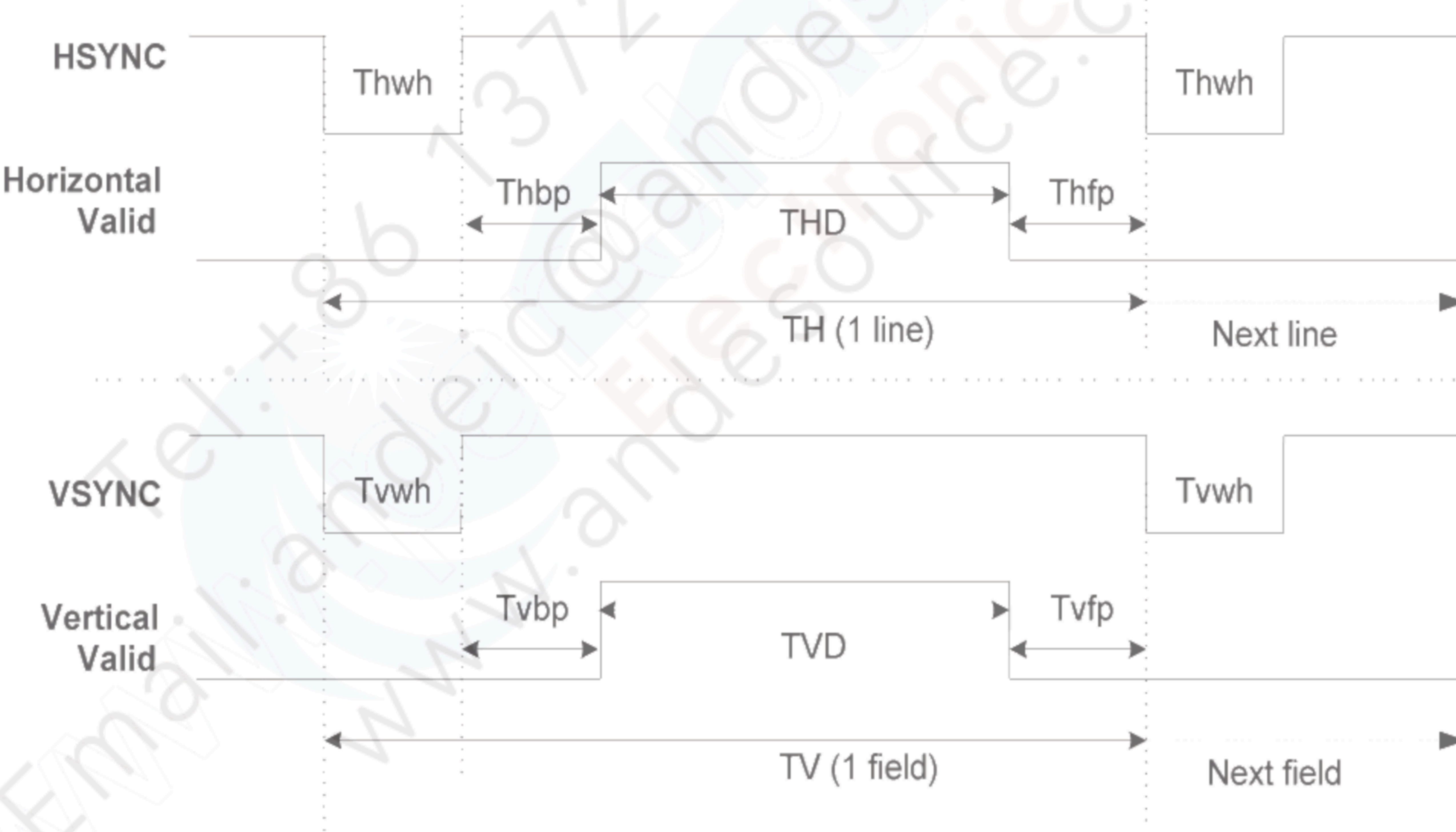
Fig.3-2 DE Mode Input Timing
