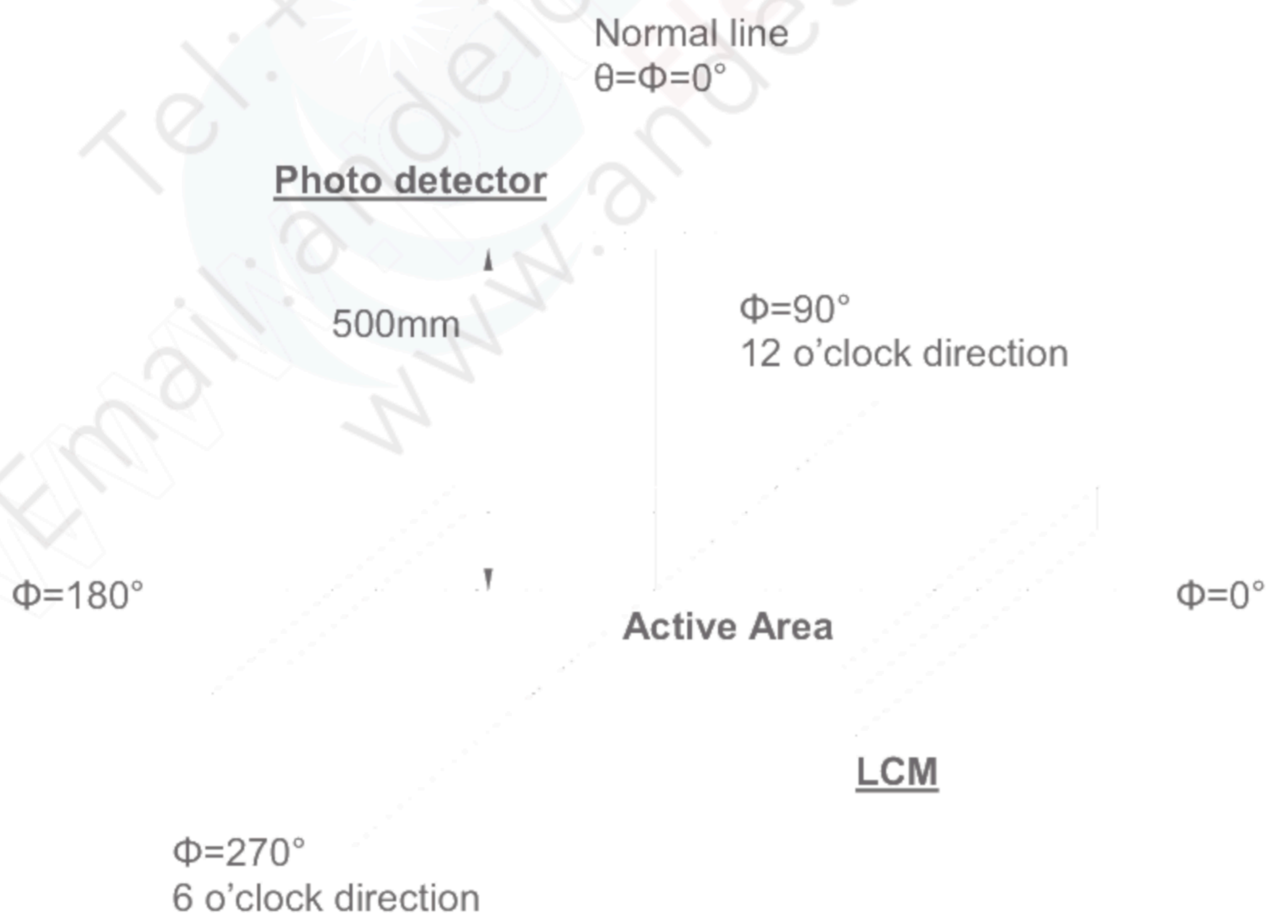
Fig. 4-2 Optical measurement system setup
