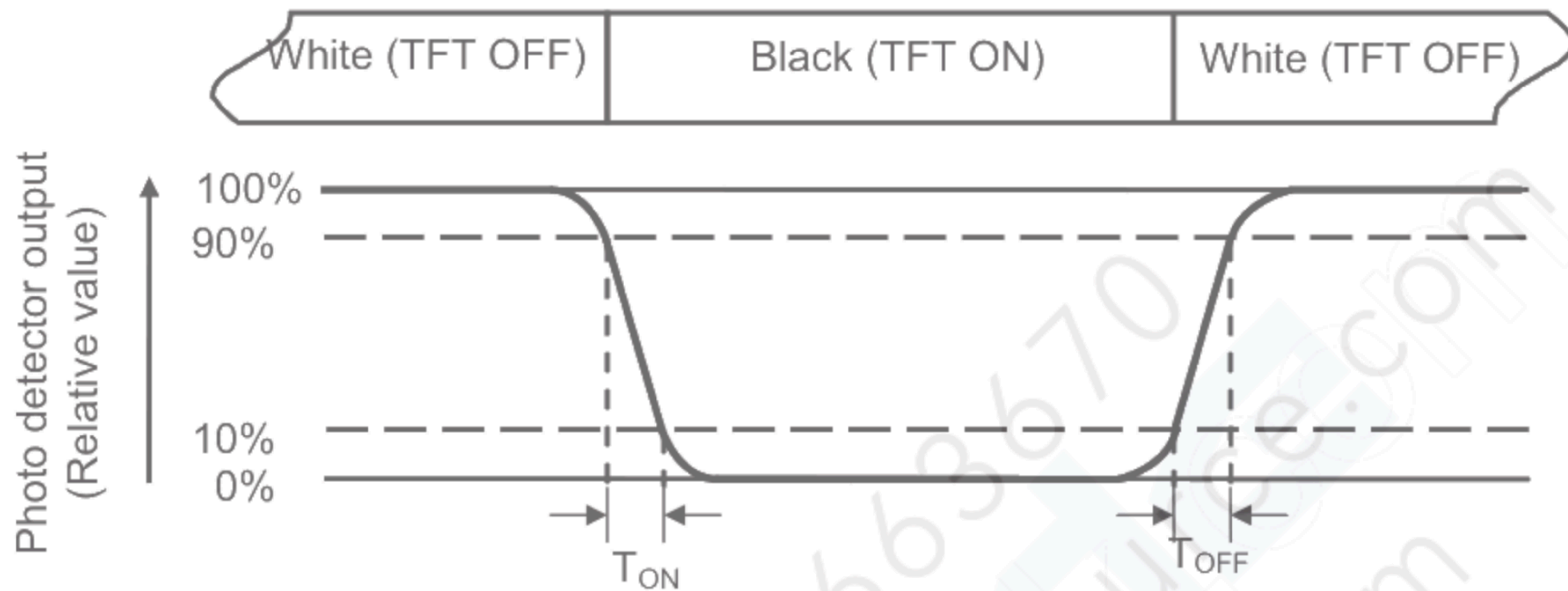
Fig. 4-3 Definition of response time
