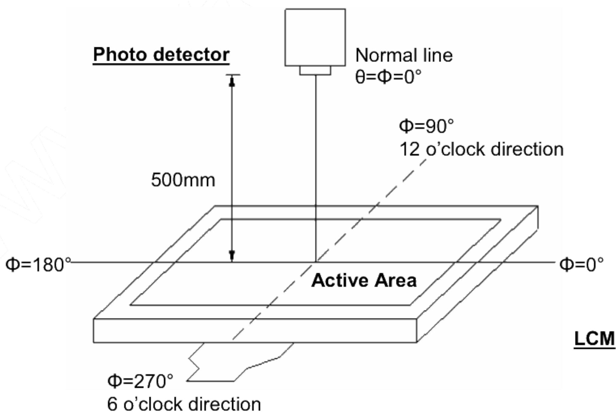
Fig. 4-2 Optical measurement system setup
