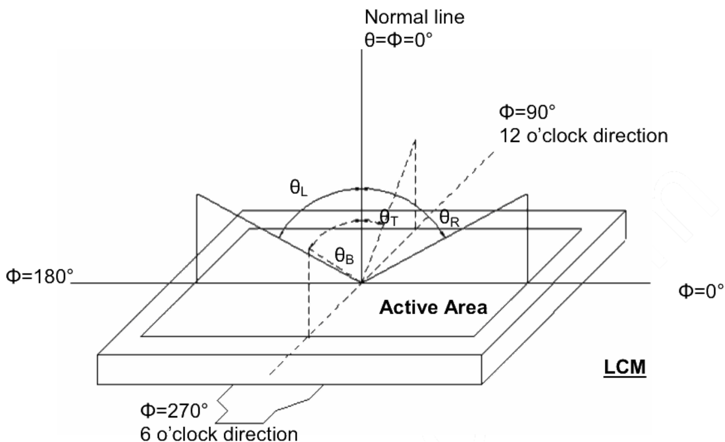
Fig. 4-1 Definition of viewing angle
