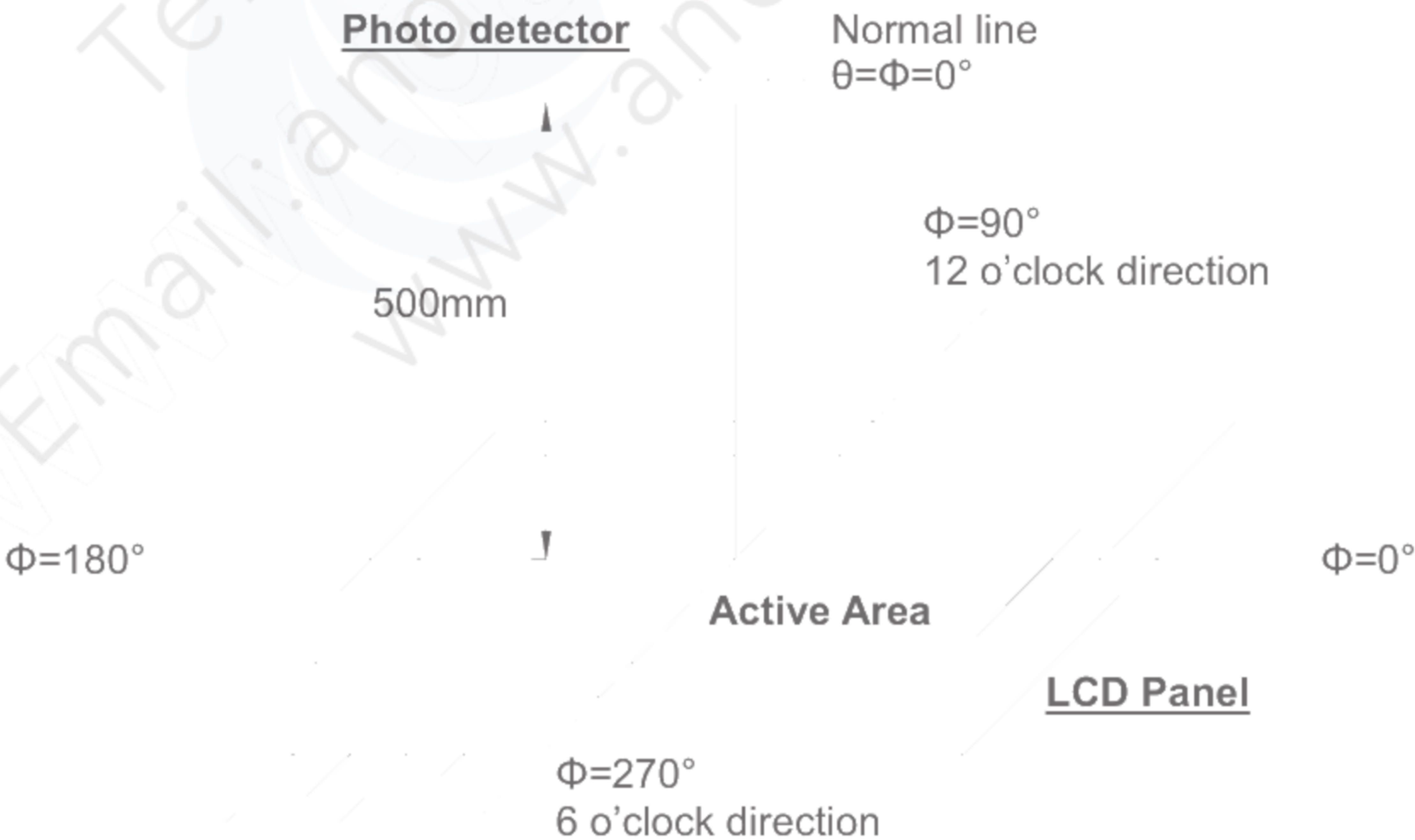
Fig. 4-2 Optical measurement system setup
