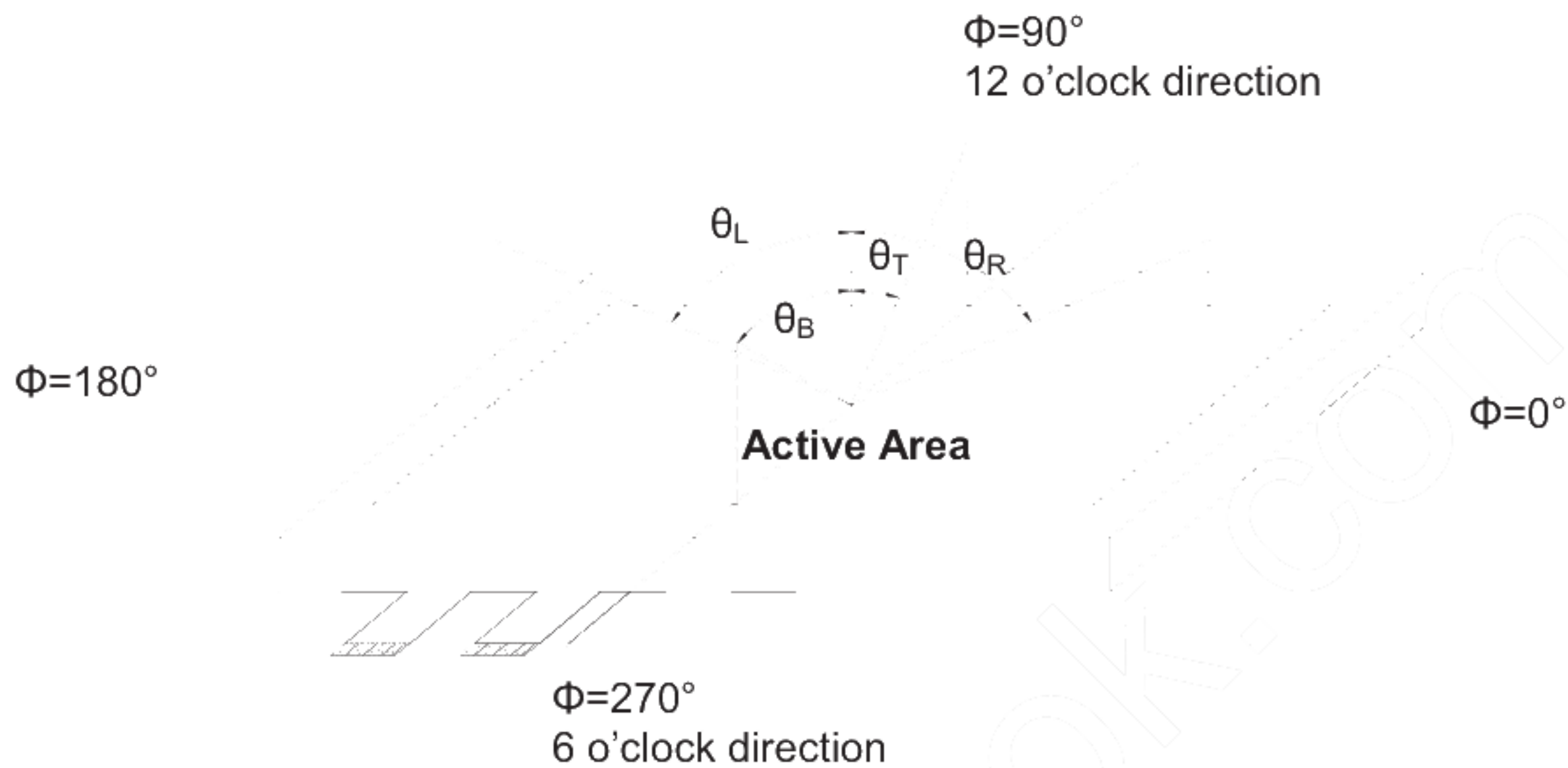
Fig. 4-1 Definition of viewing angle
