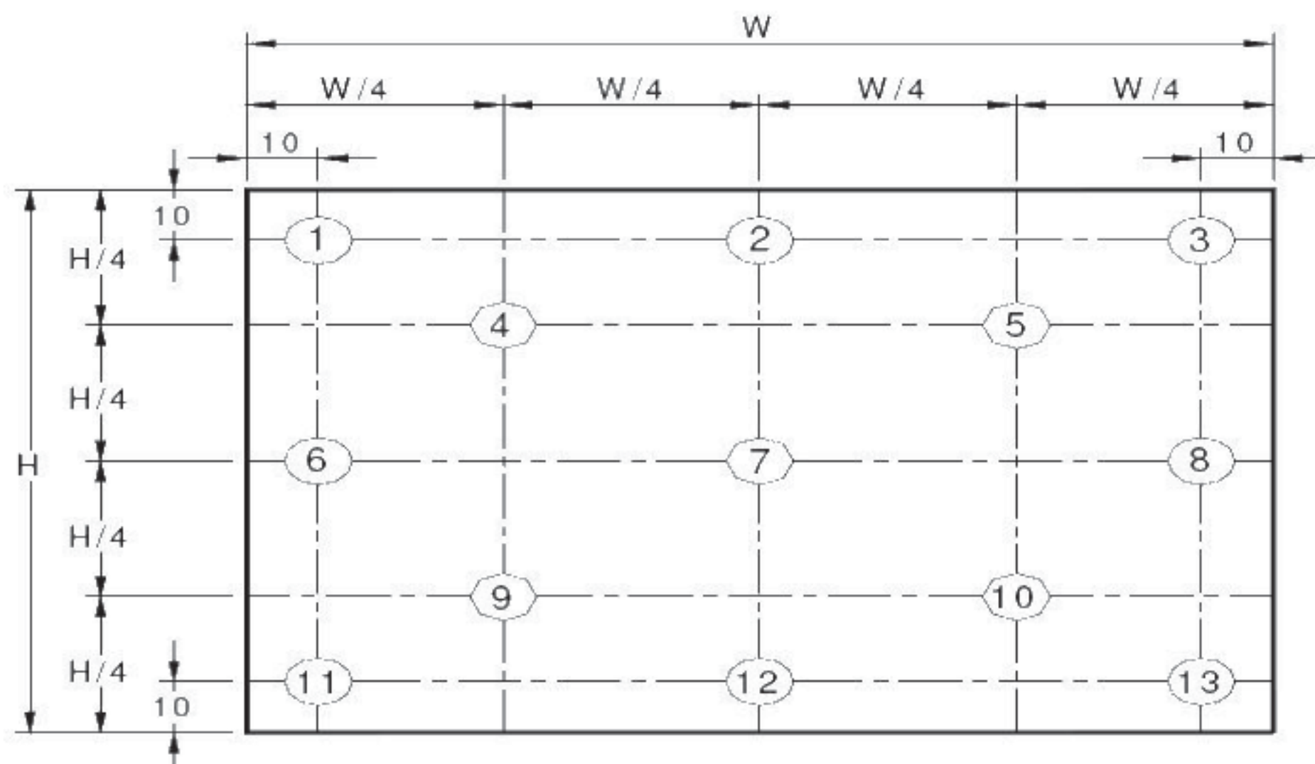
Figure 3. Uniformity Measurement Locations (13 points)
