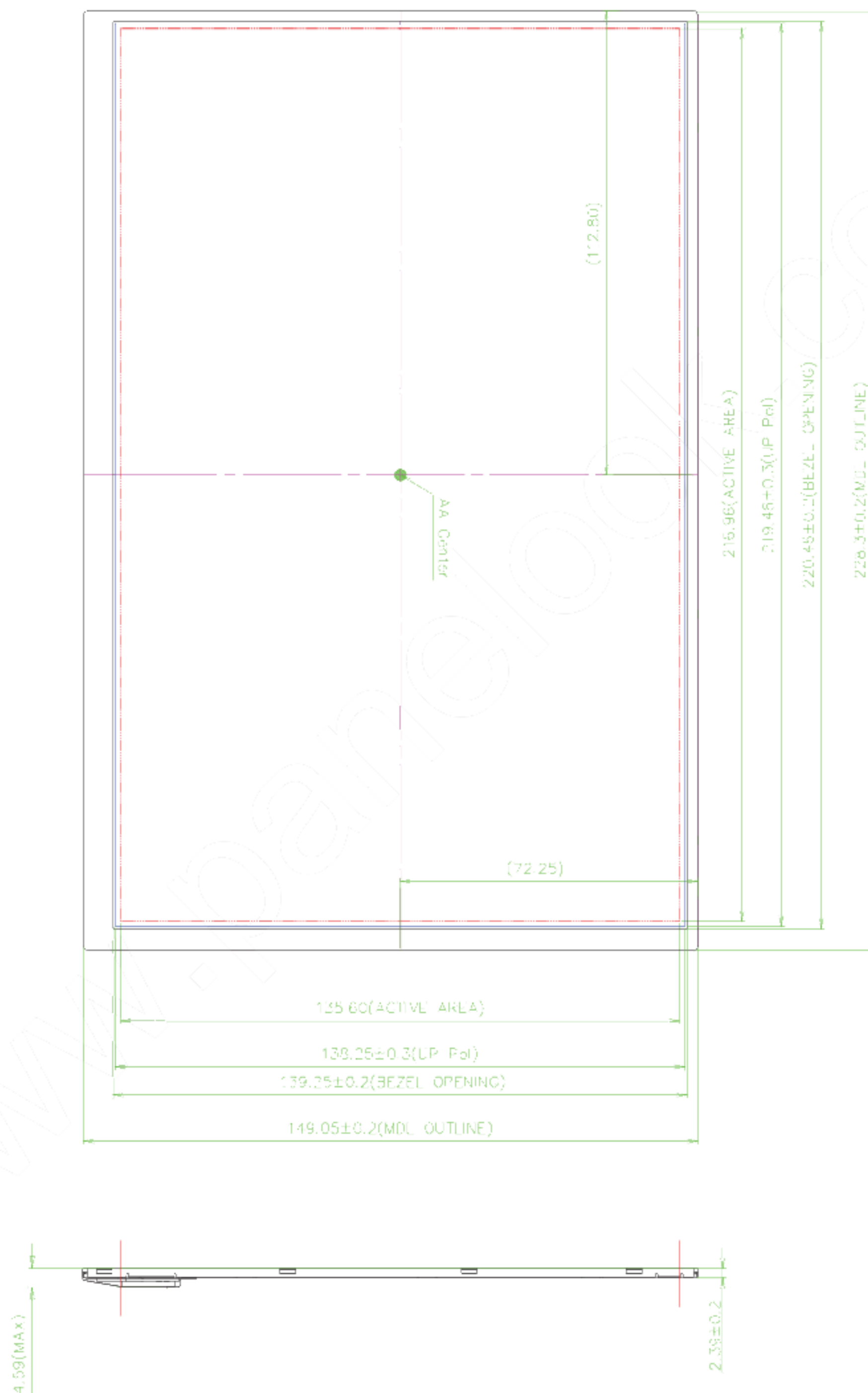
Figure 6. TFT-LCD Module Outline Dimension (Front View)
