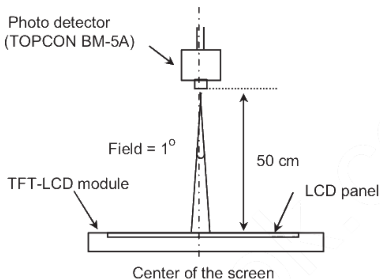
Figure 1. Measurement Set Up
