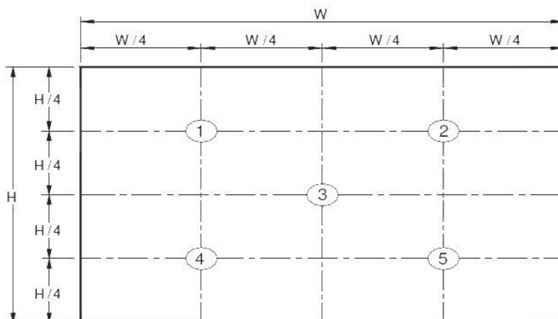
Figure 2. White Luminance and Uniformity Measurement Locations (5 points)
