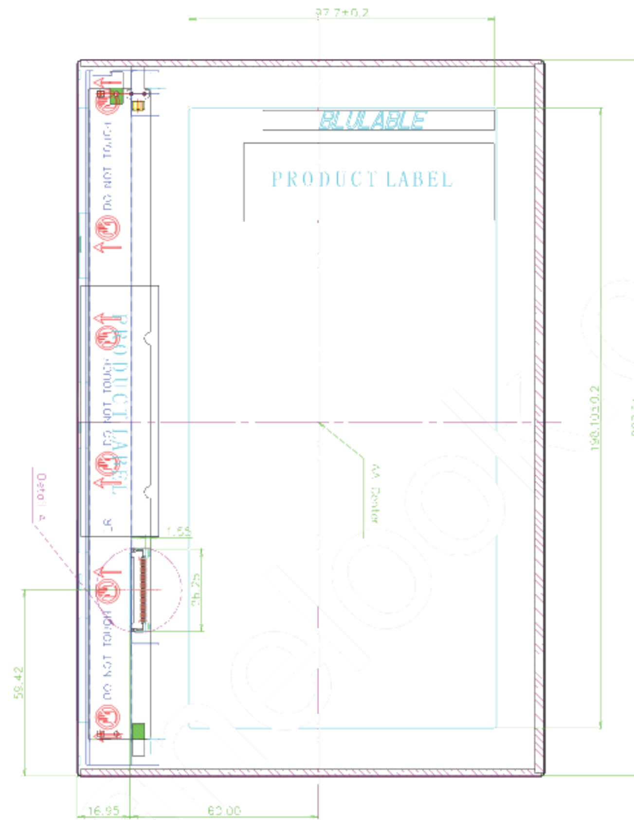
Figure 7. TFT-LCD Module Outline Dimensions (Rear view)
