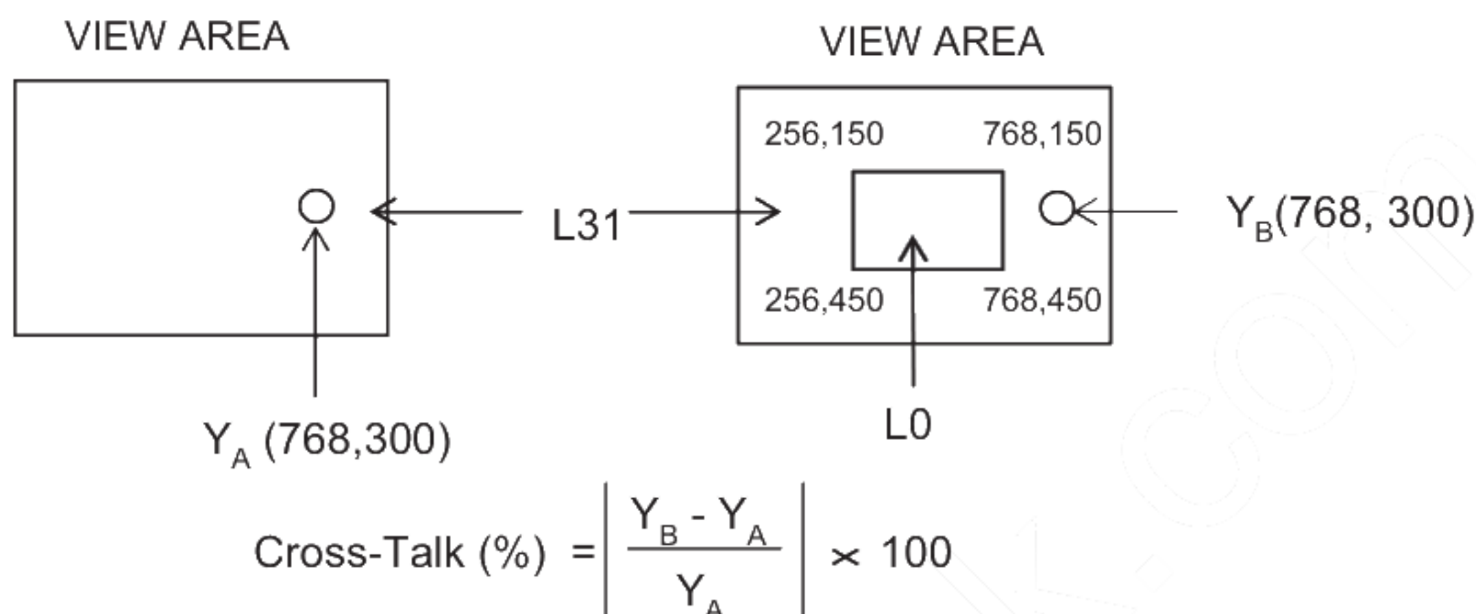
Figure 5. Cross Modulation Test Description
