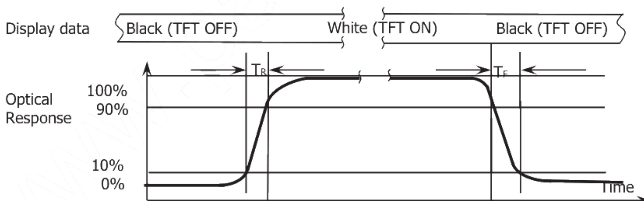
Figure 4. Response Time Testing
