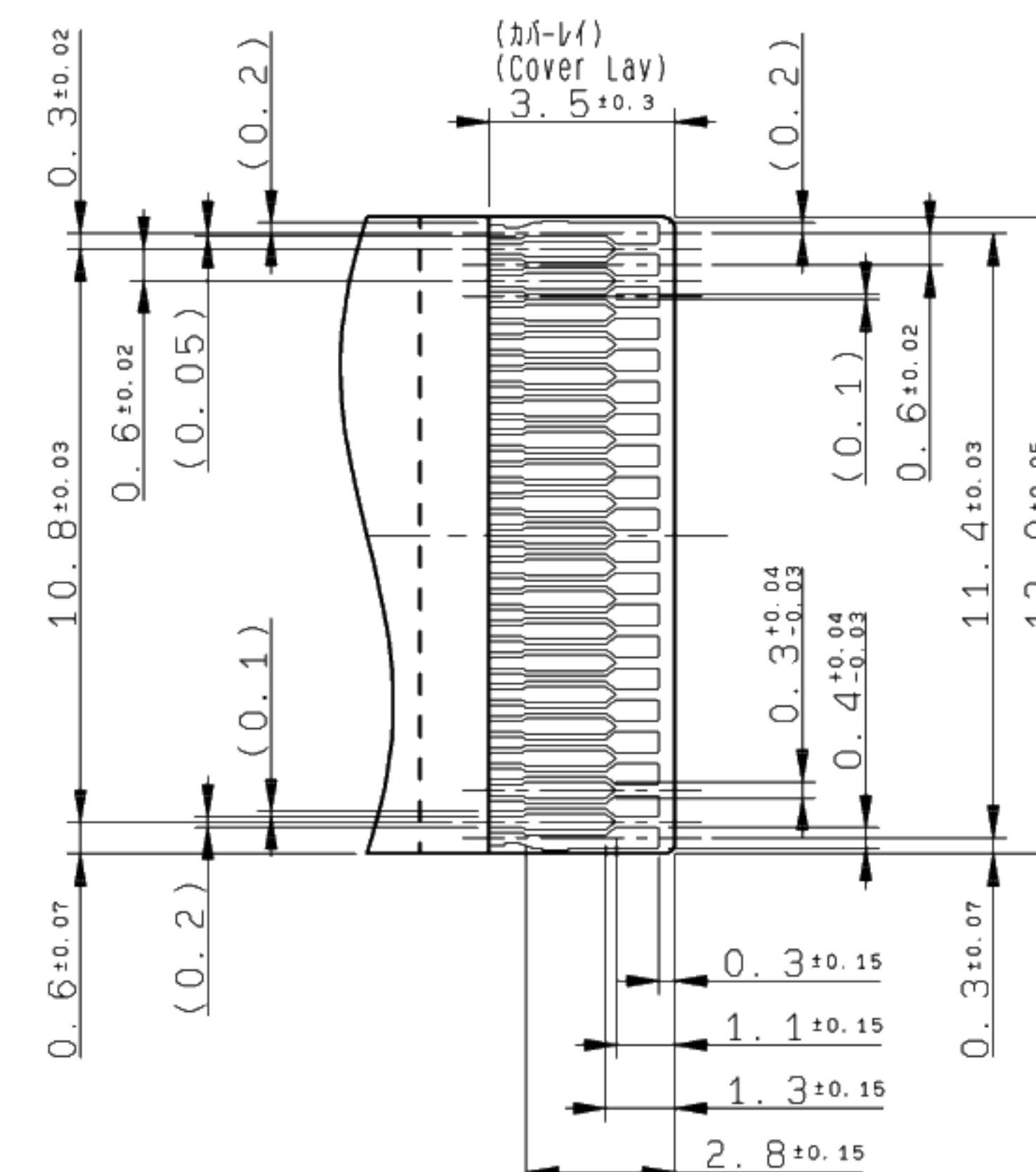
Detail A (S=5/1)
