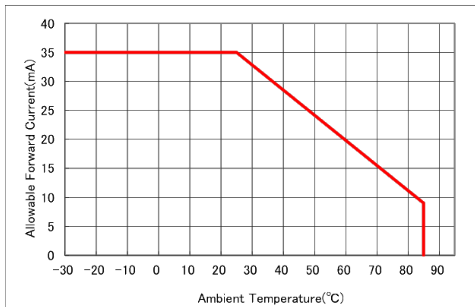
Fig. 2: Allowable Forward Current
