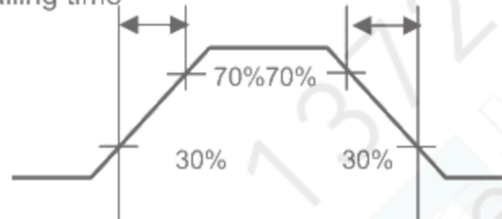
Signal rising and falling time
