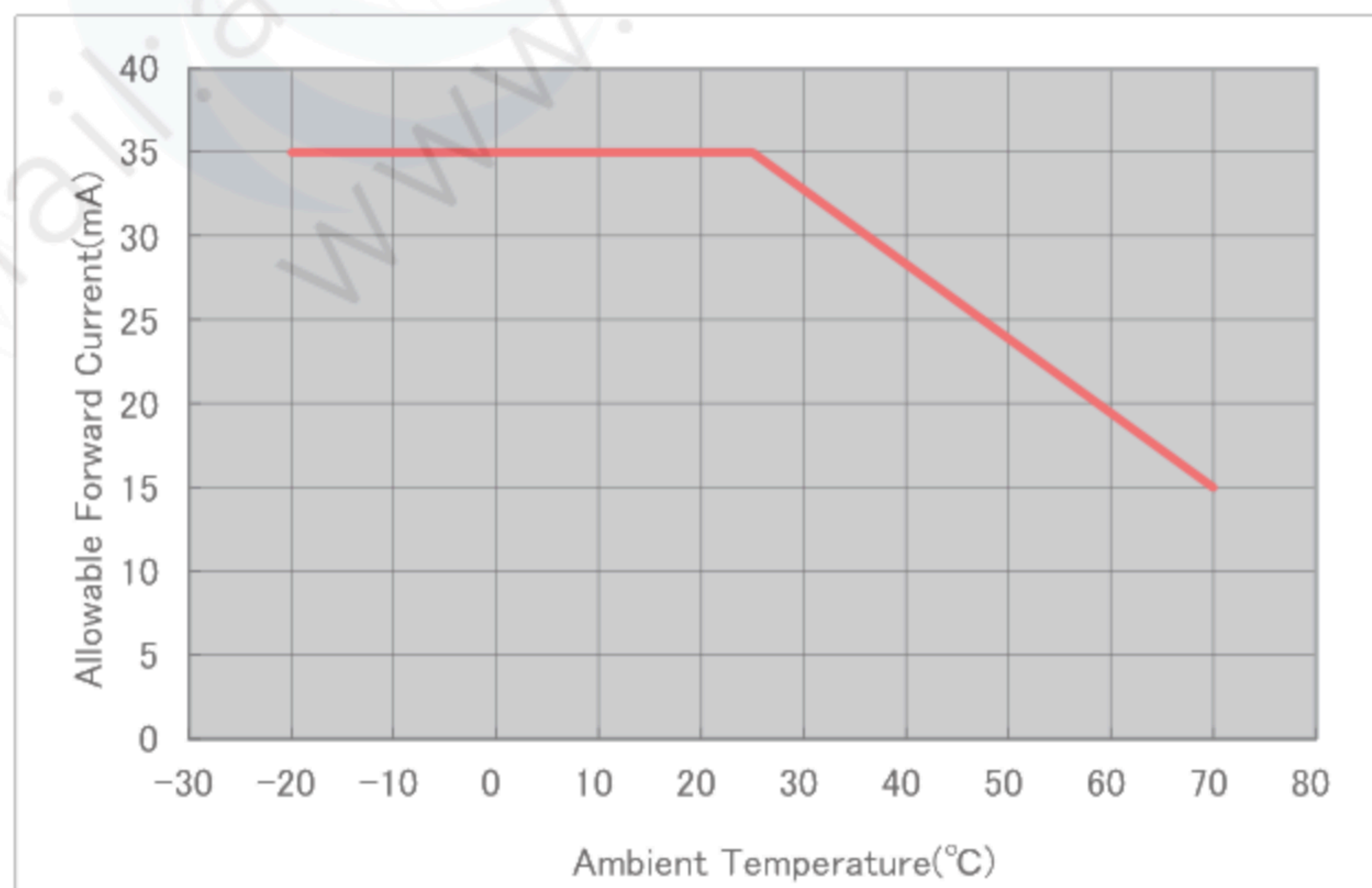
Fig. 1: Allowable Forward Current
