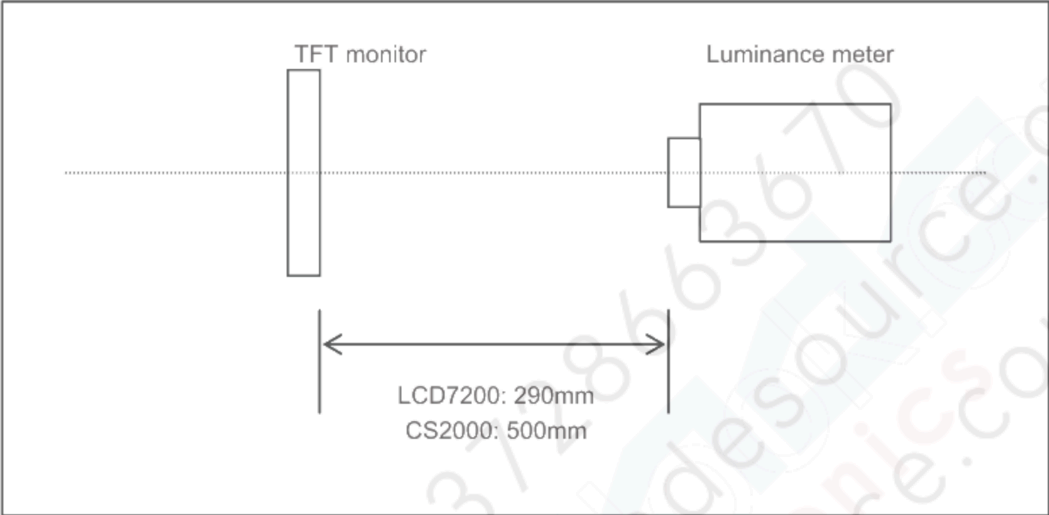
Dark box at constant temperature
