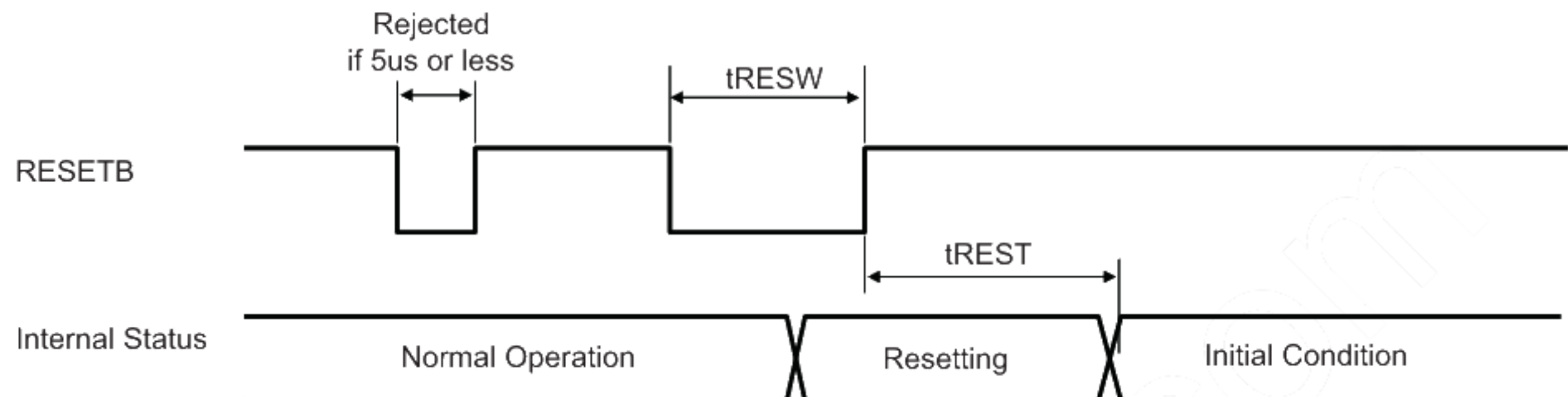
Fig.F RESETB input timing
