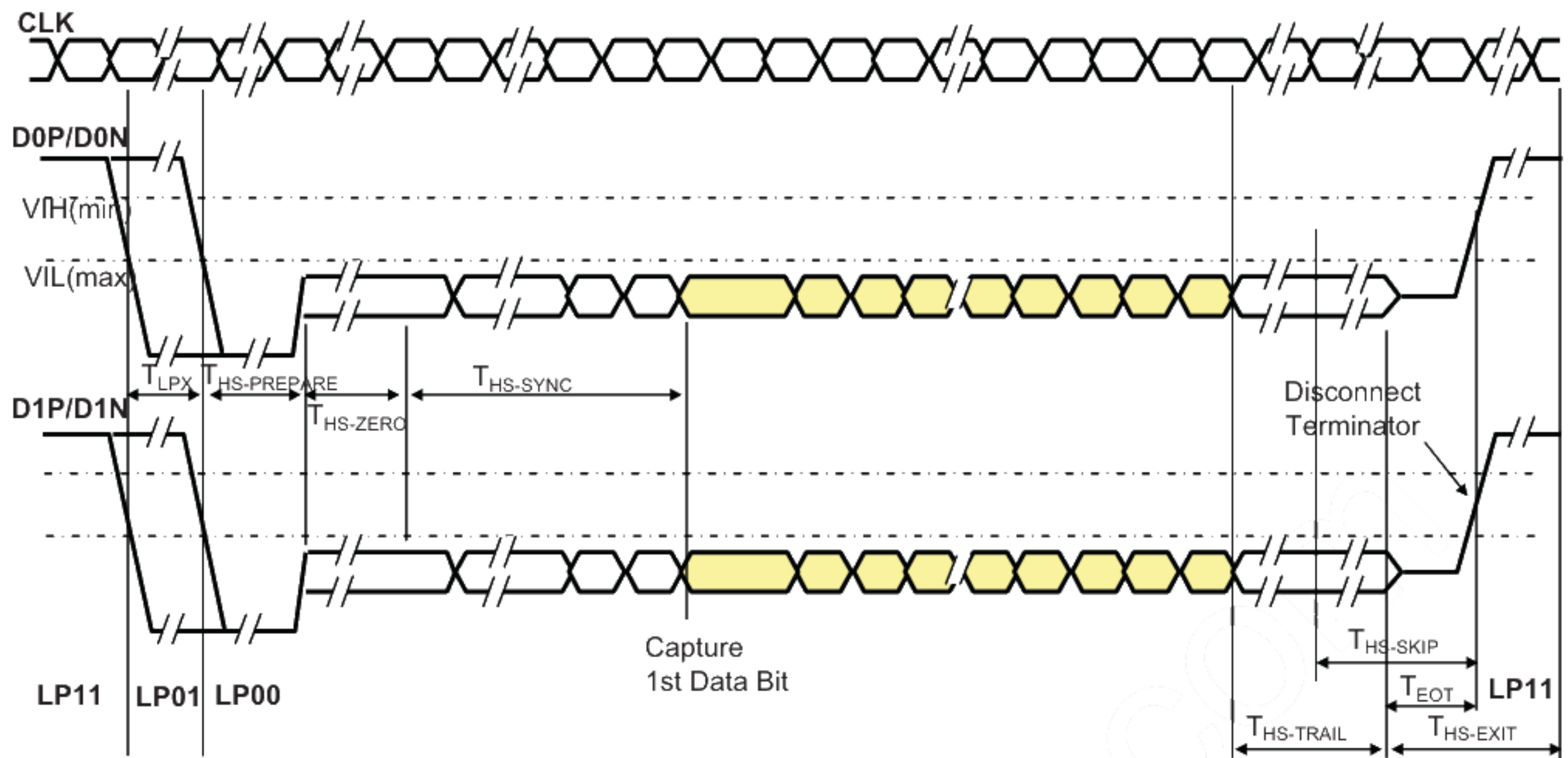
Fig.C HS Data Transmission in Bursts
