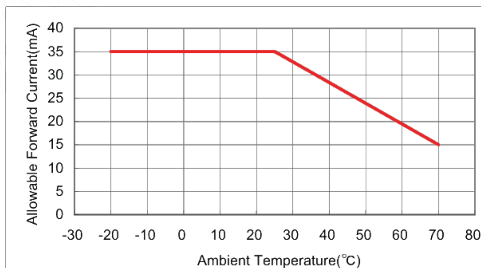
Fig. 2: Allowable Forward Current
