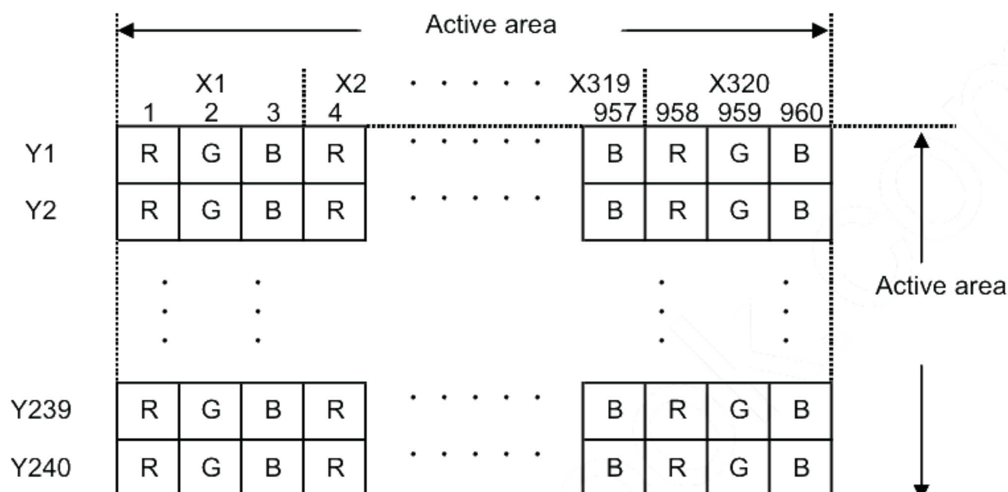
Fig. 1: Dot arrangement (FPC cable placed down)
