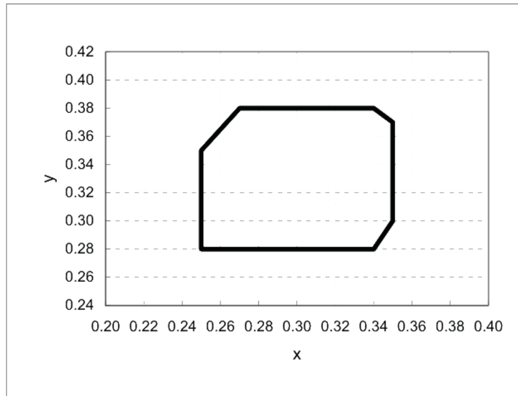
White Chromaticity Range
