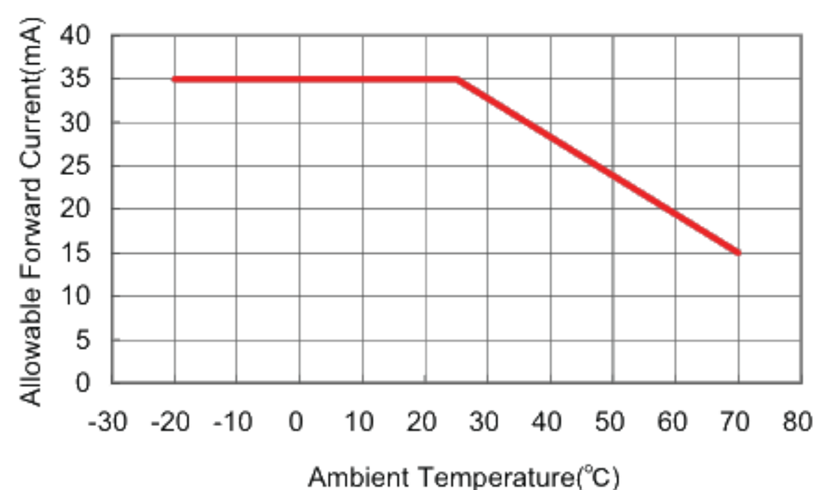
Fig. 2: Allowable Forward Current
