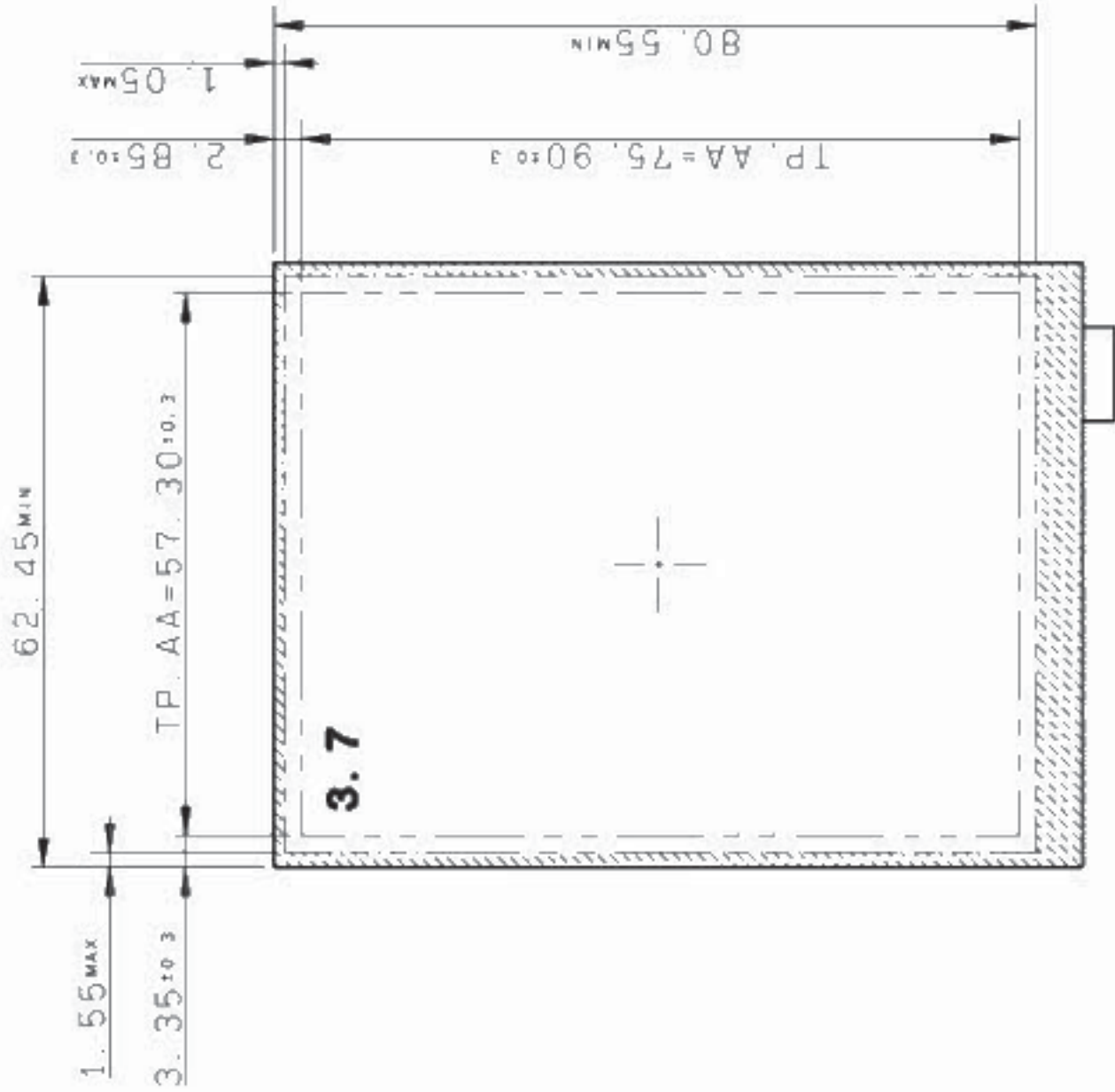
Cusion area (Touchpanel) (S=1/1)
