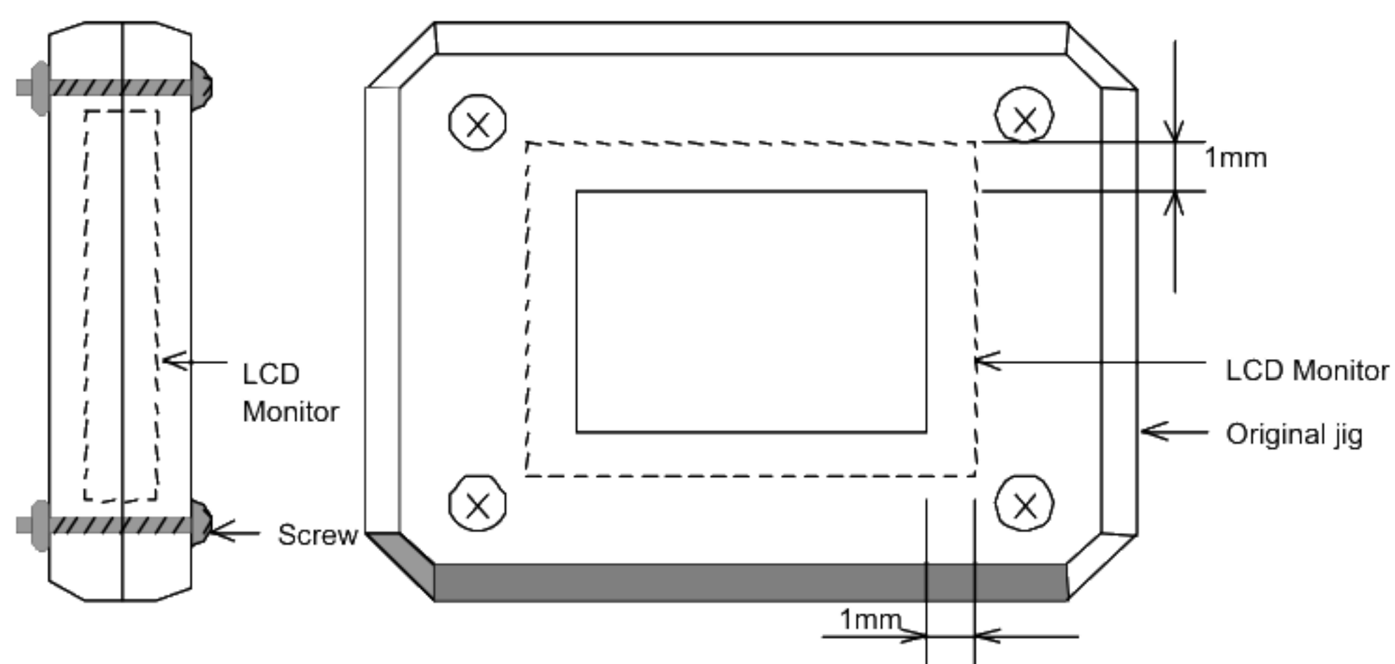
ORTUS TECHNOLOGY Original Jig
