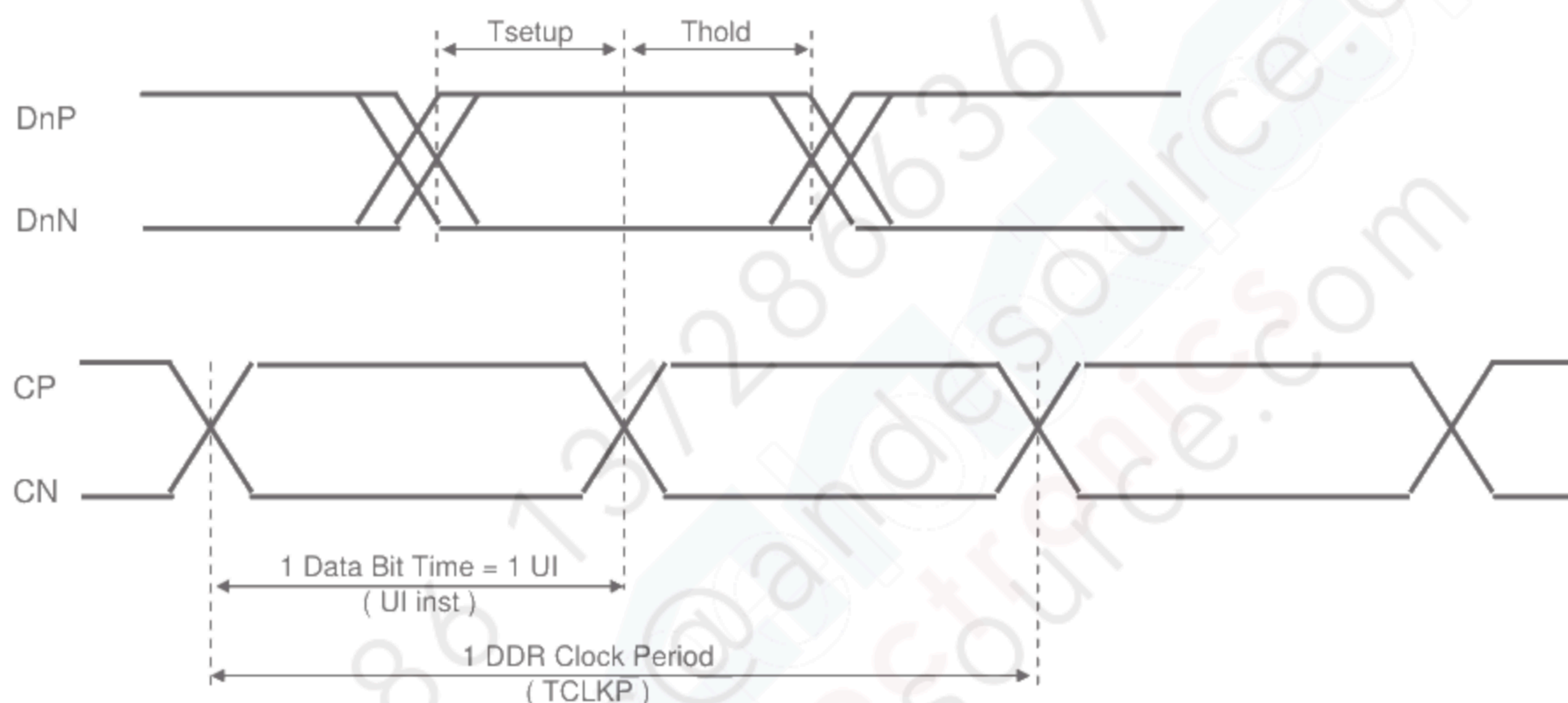
Fig.B Data to Clock Timing Definitions
