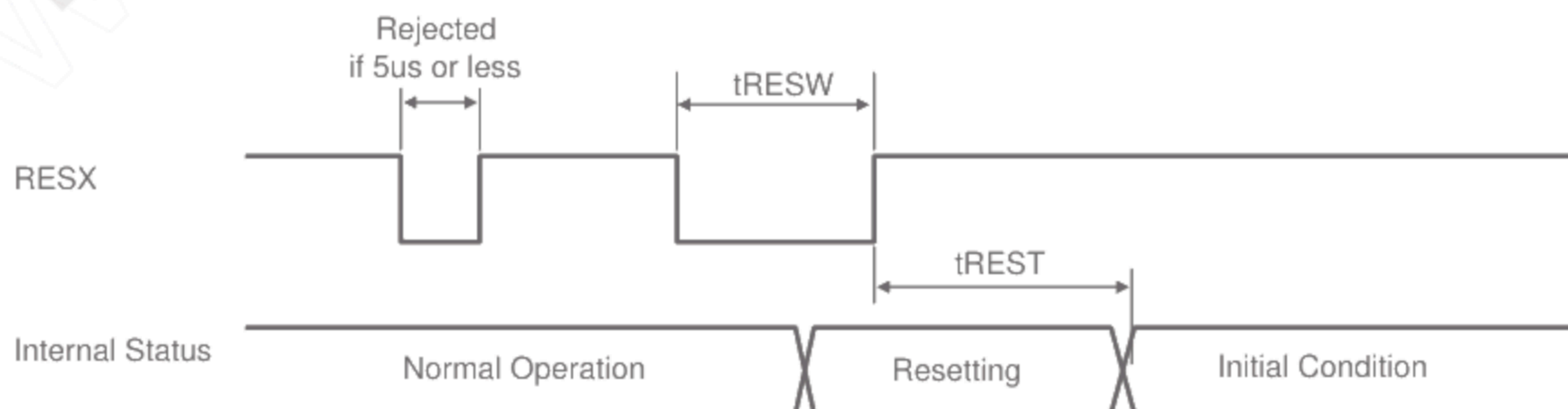
Fig.D RESX input timing
