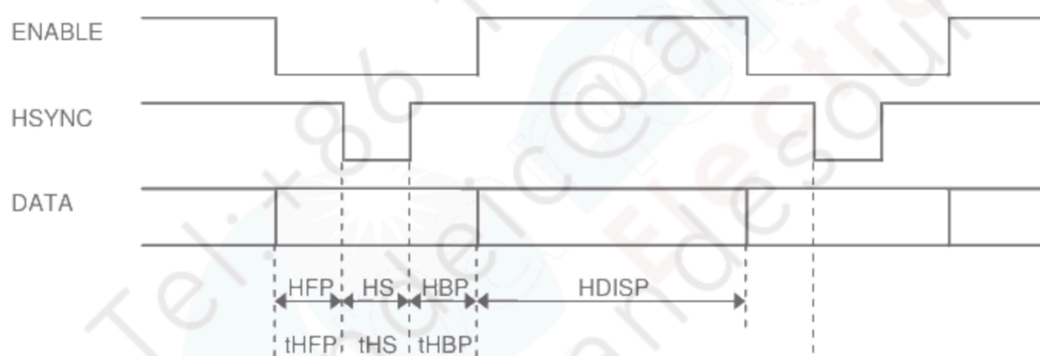
Fig.C Vertical ,Horizontal timing
