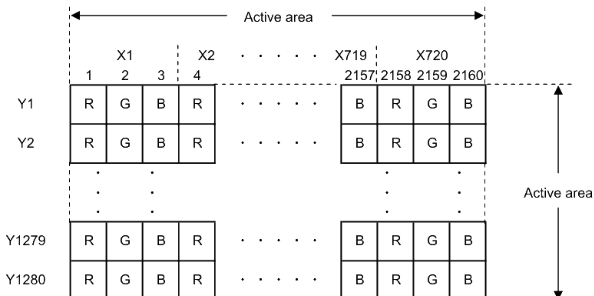
Fig.1 Dot arrangement (FPC cable placed lower right )
