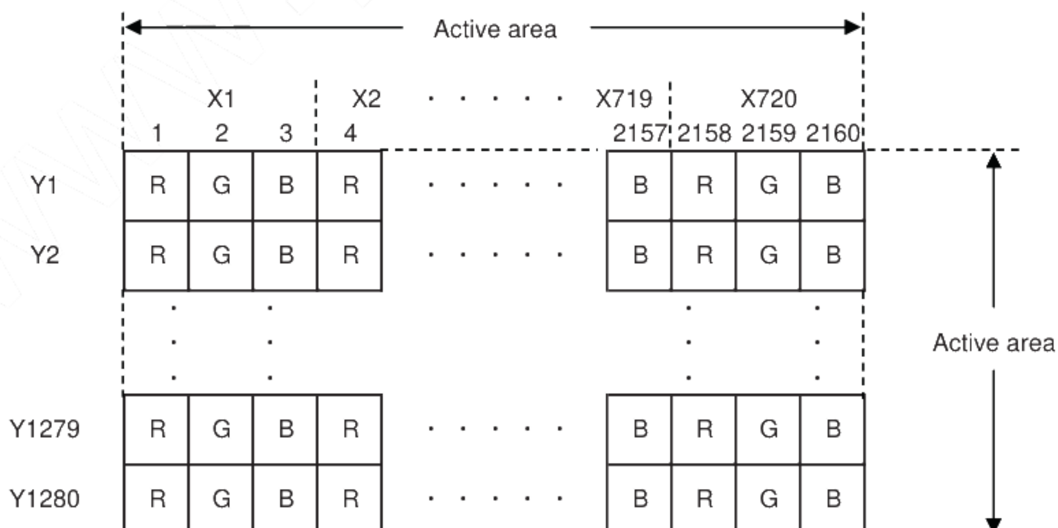
Dot arrangement (FPC cable placed)
