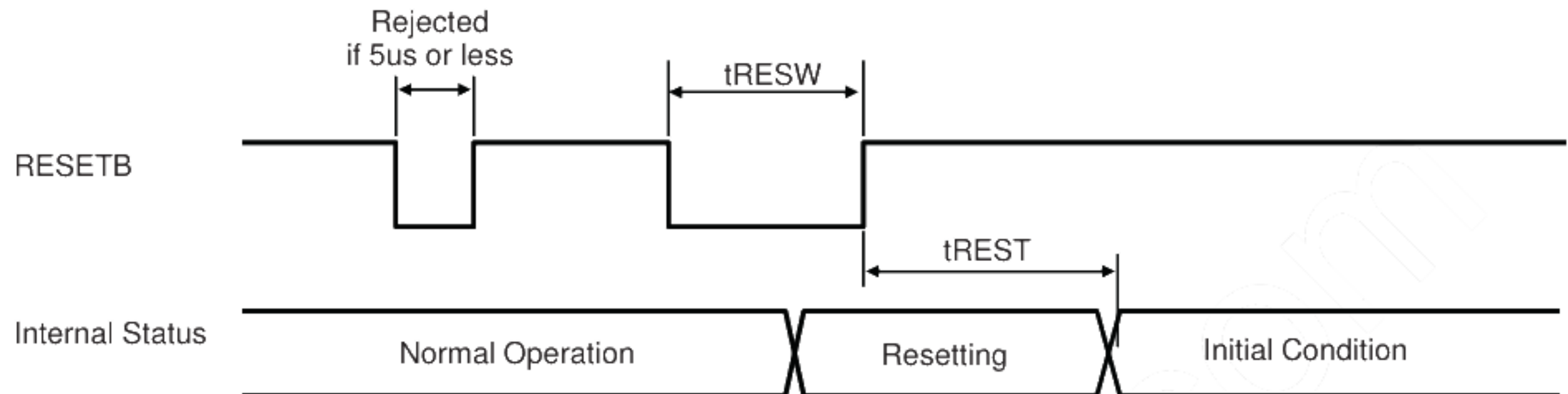
RESETB input timing
