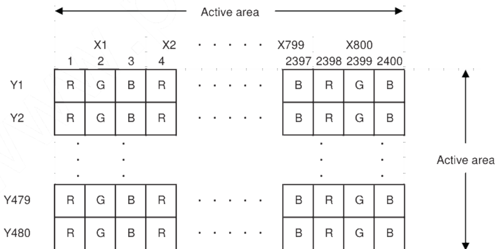
Dot arrangement (FPC cable placed down side)
