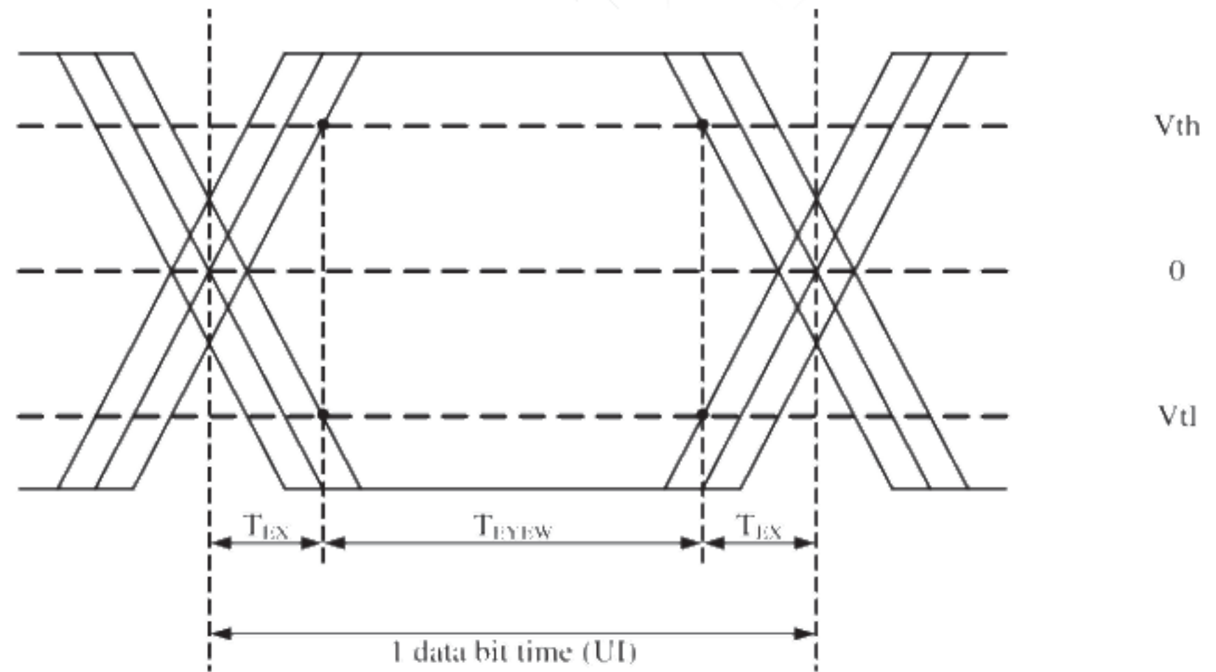
LVDS input eye diagram
