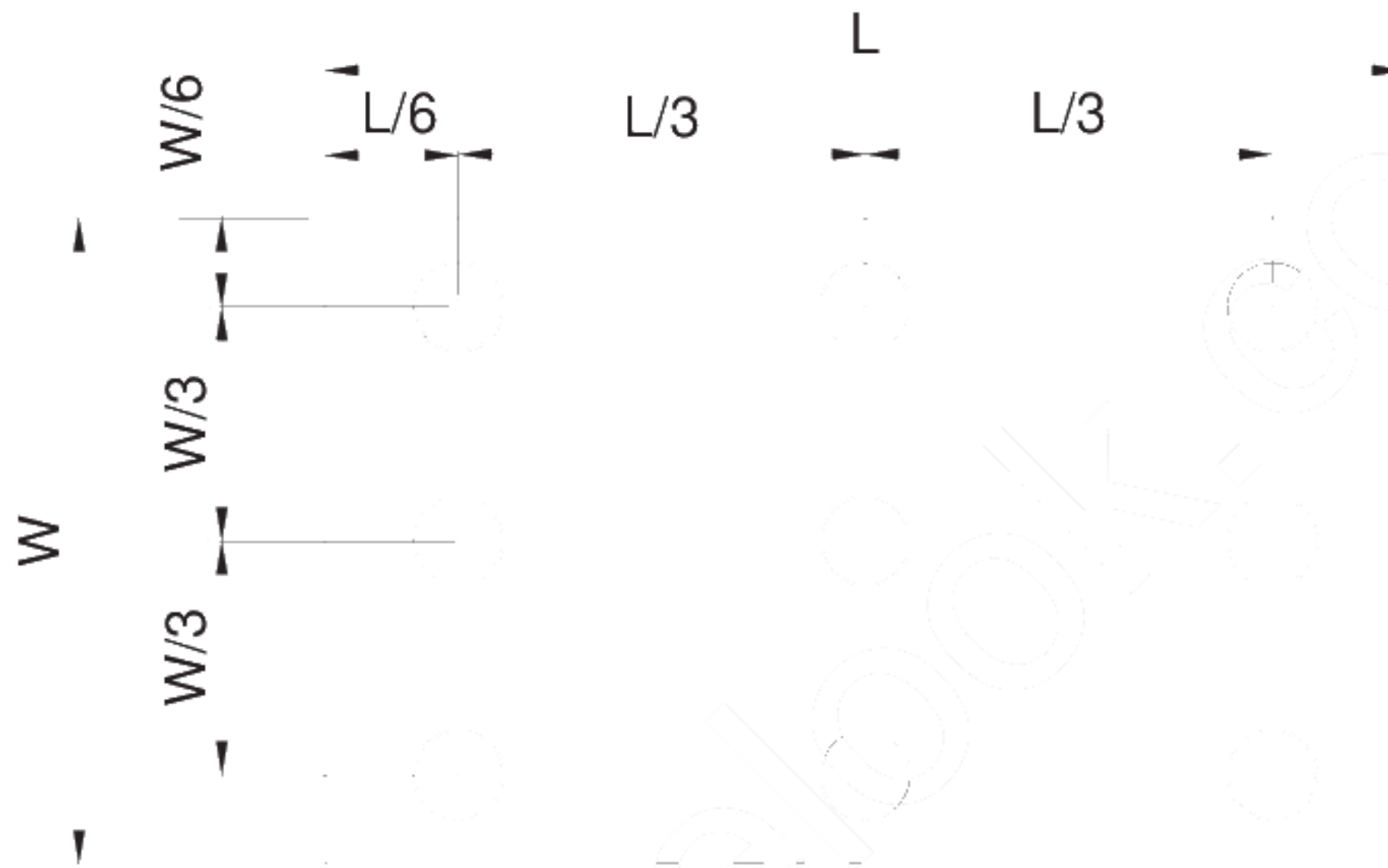
Fig. 4-4 Definition of measuring points
