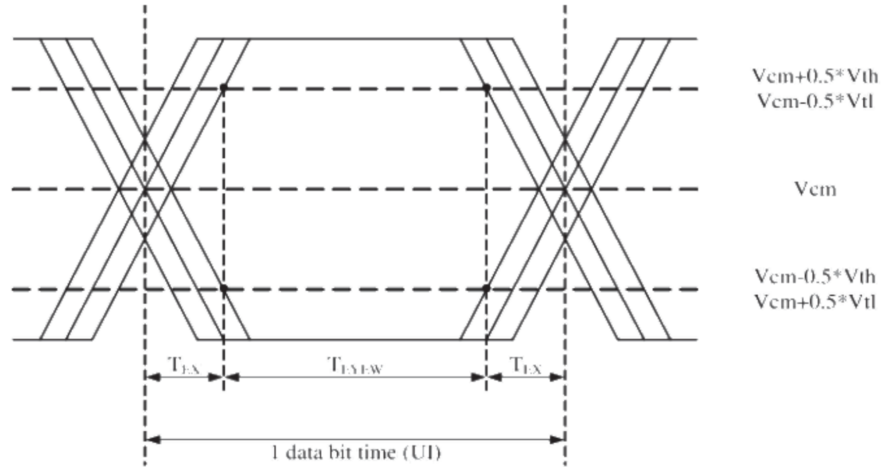
LVDS input eye diagram
