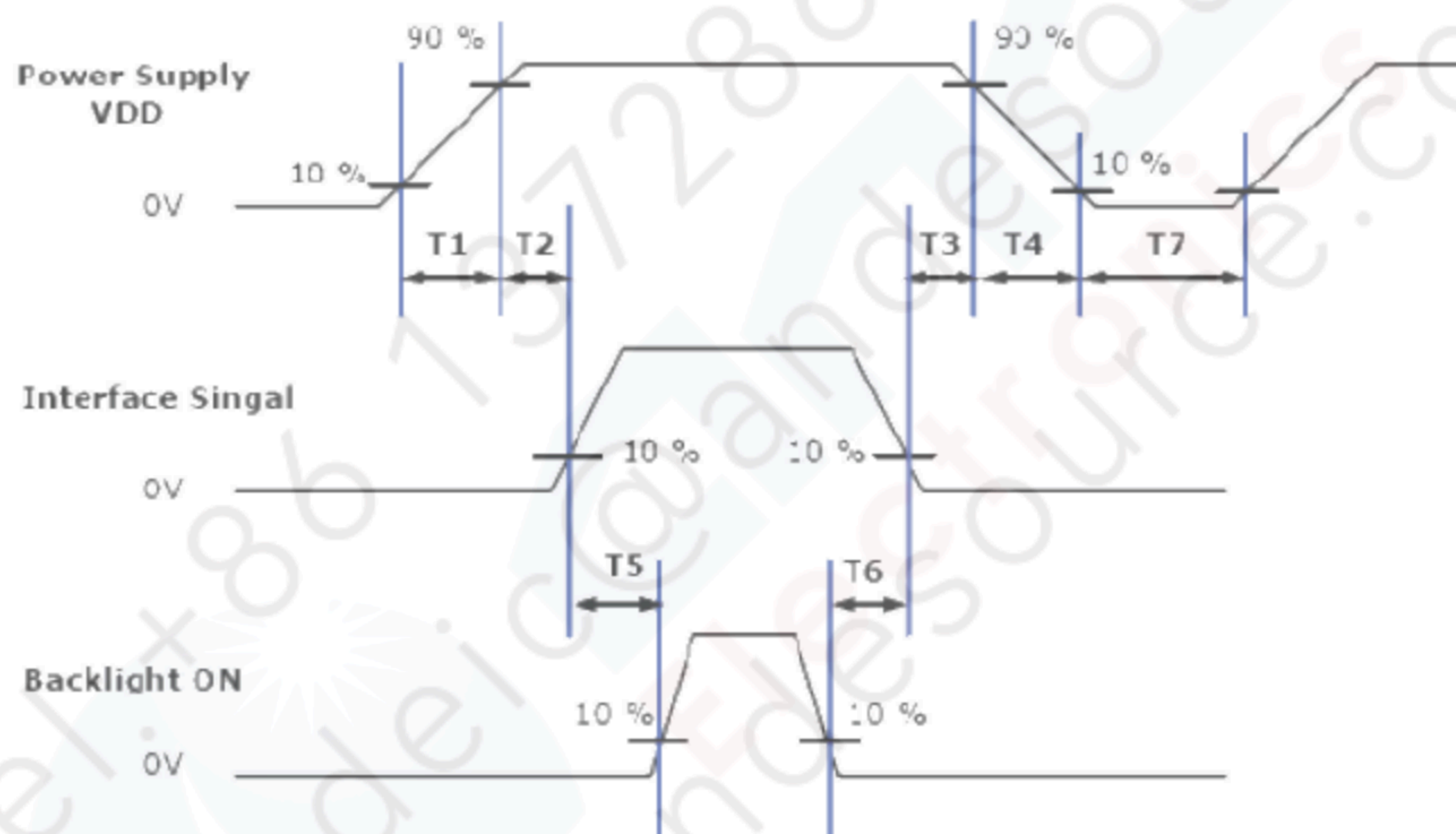
Power ON/OFF sequence timing
