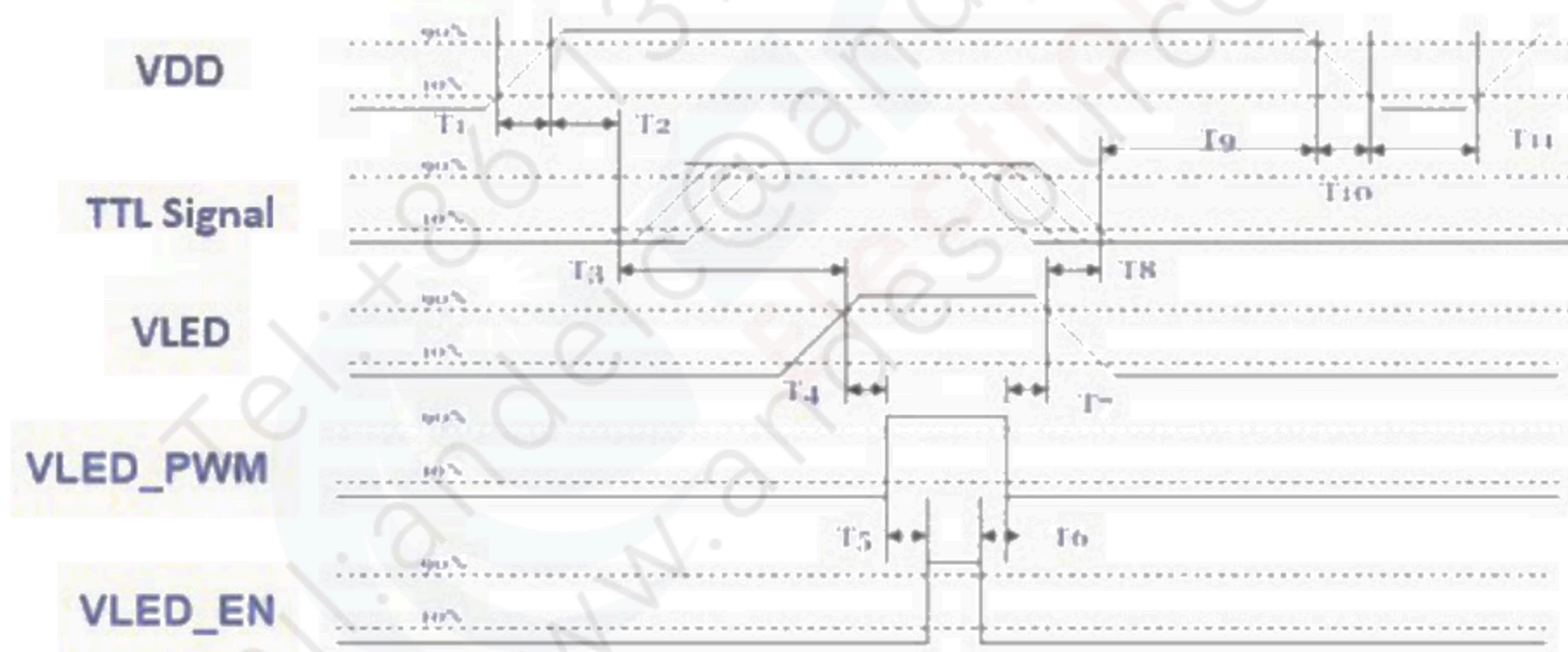
Power ON/OFF sequence timing
