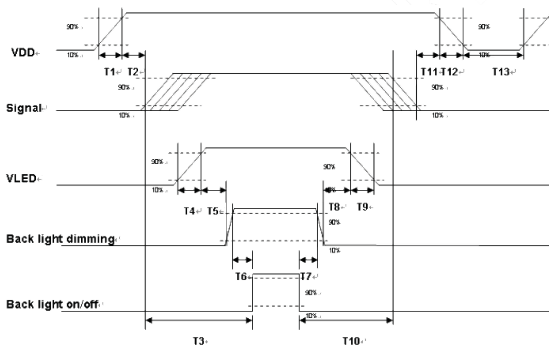
Power ON/OFF sequence timing
