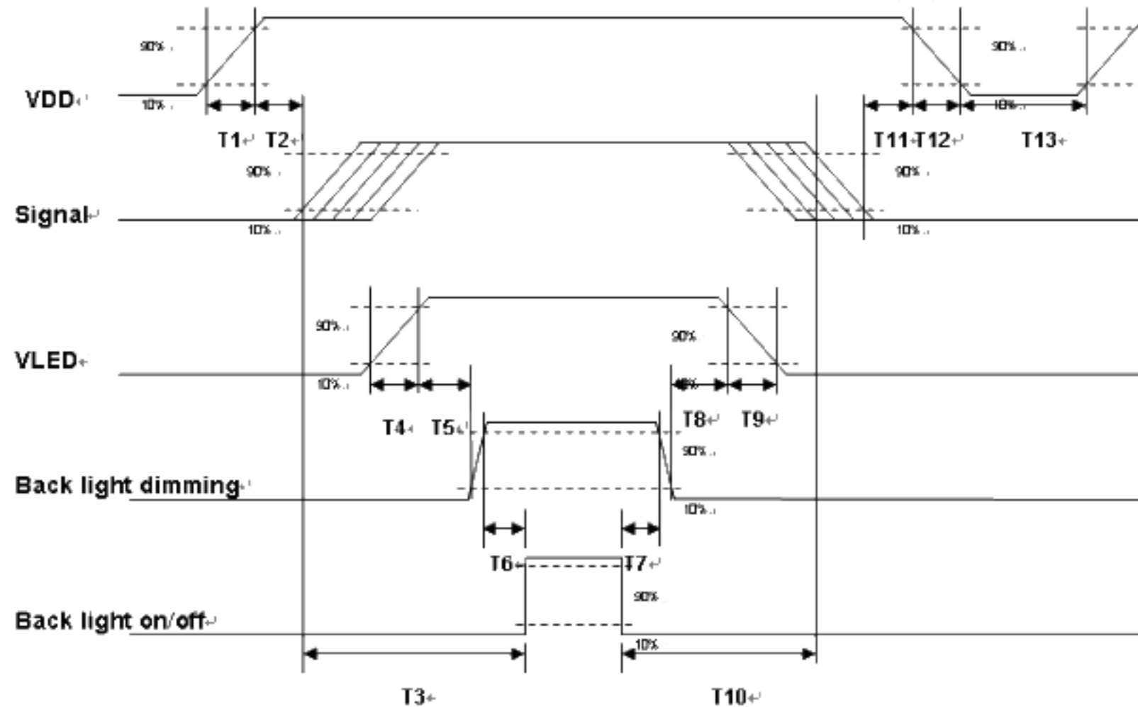
Power ON/OFF sequence timing
