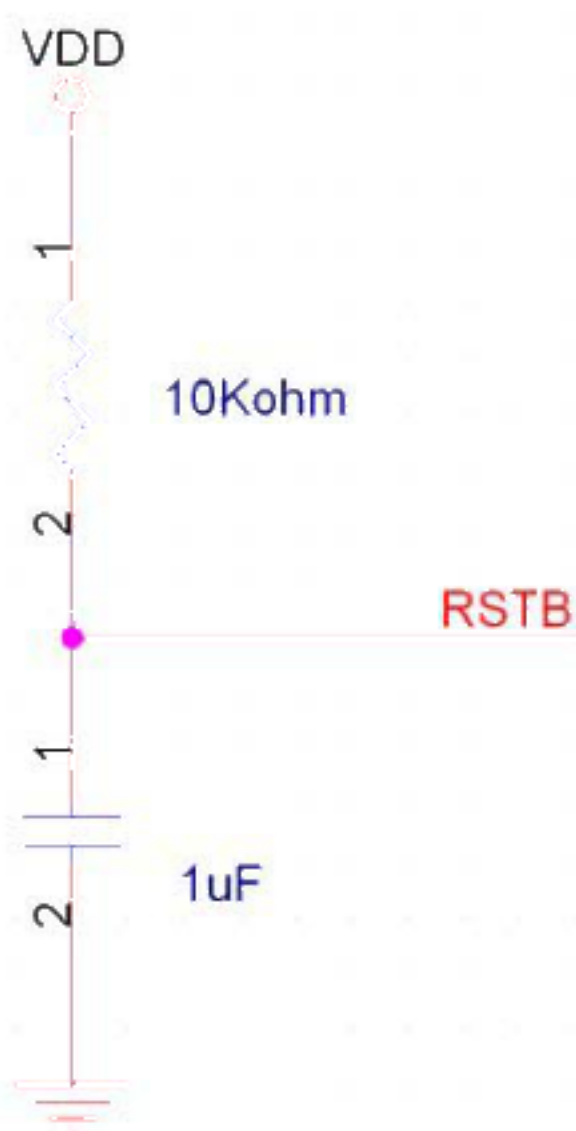
Fig. 6-3 Active Low
