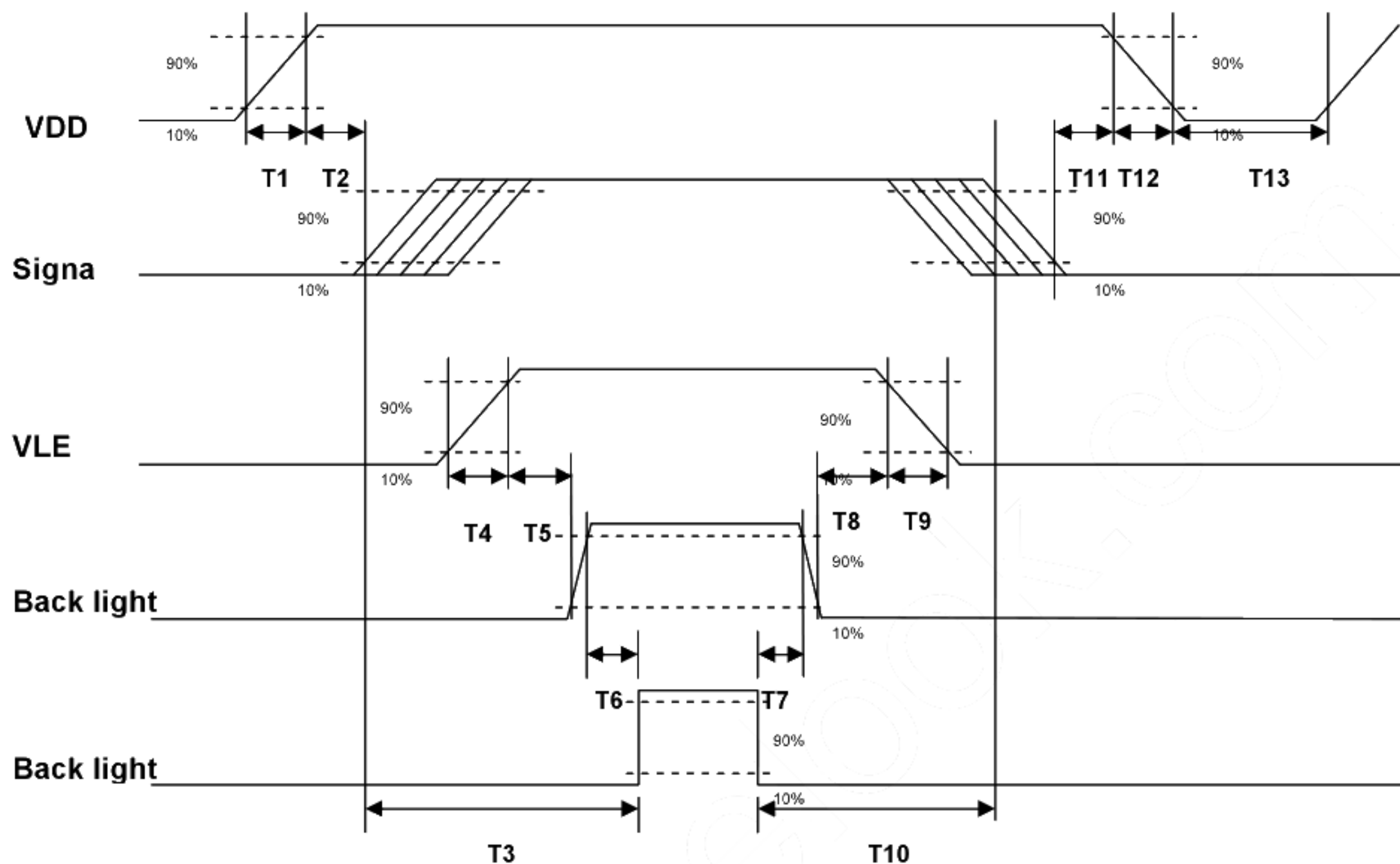
Power ON/OFF sequence timing
