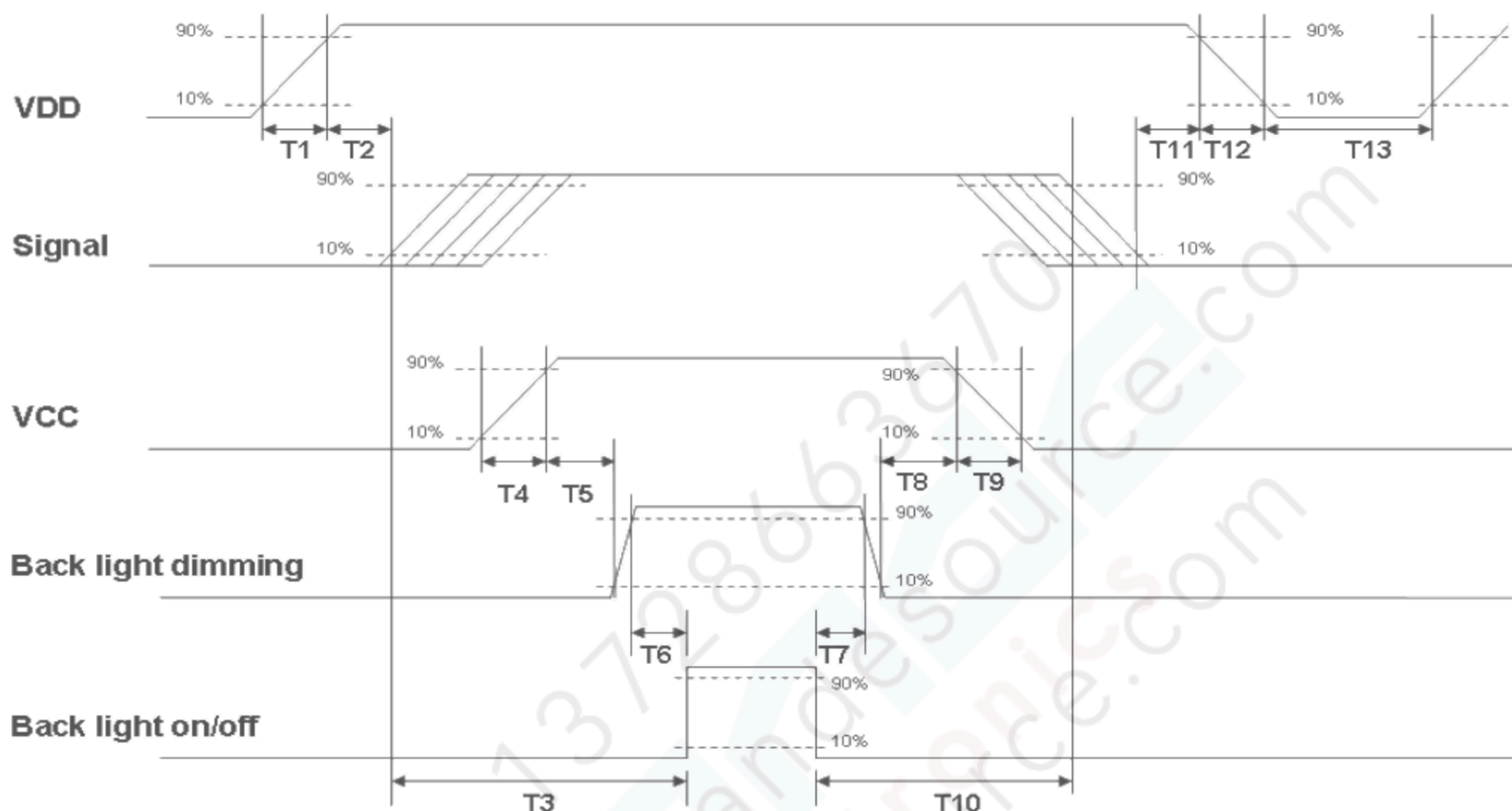
Power ON/OFF sequence timing
