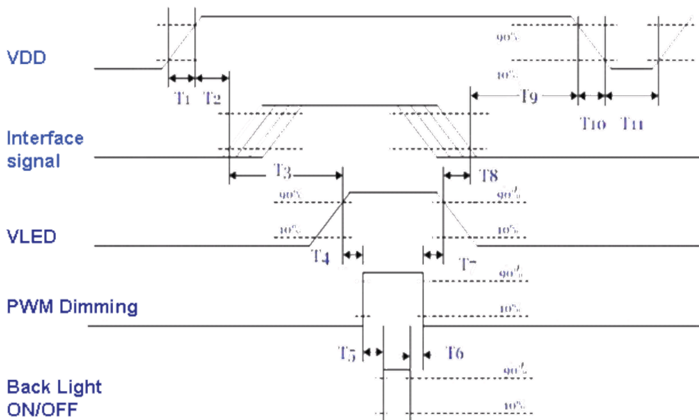
Power ON/OFF sequence timing
