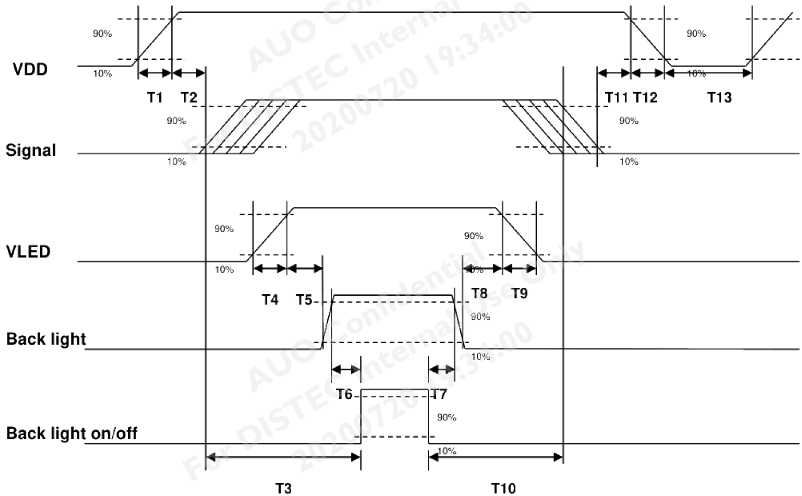
Power Sequence Timing
