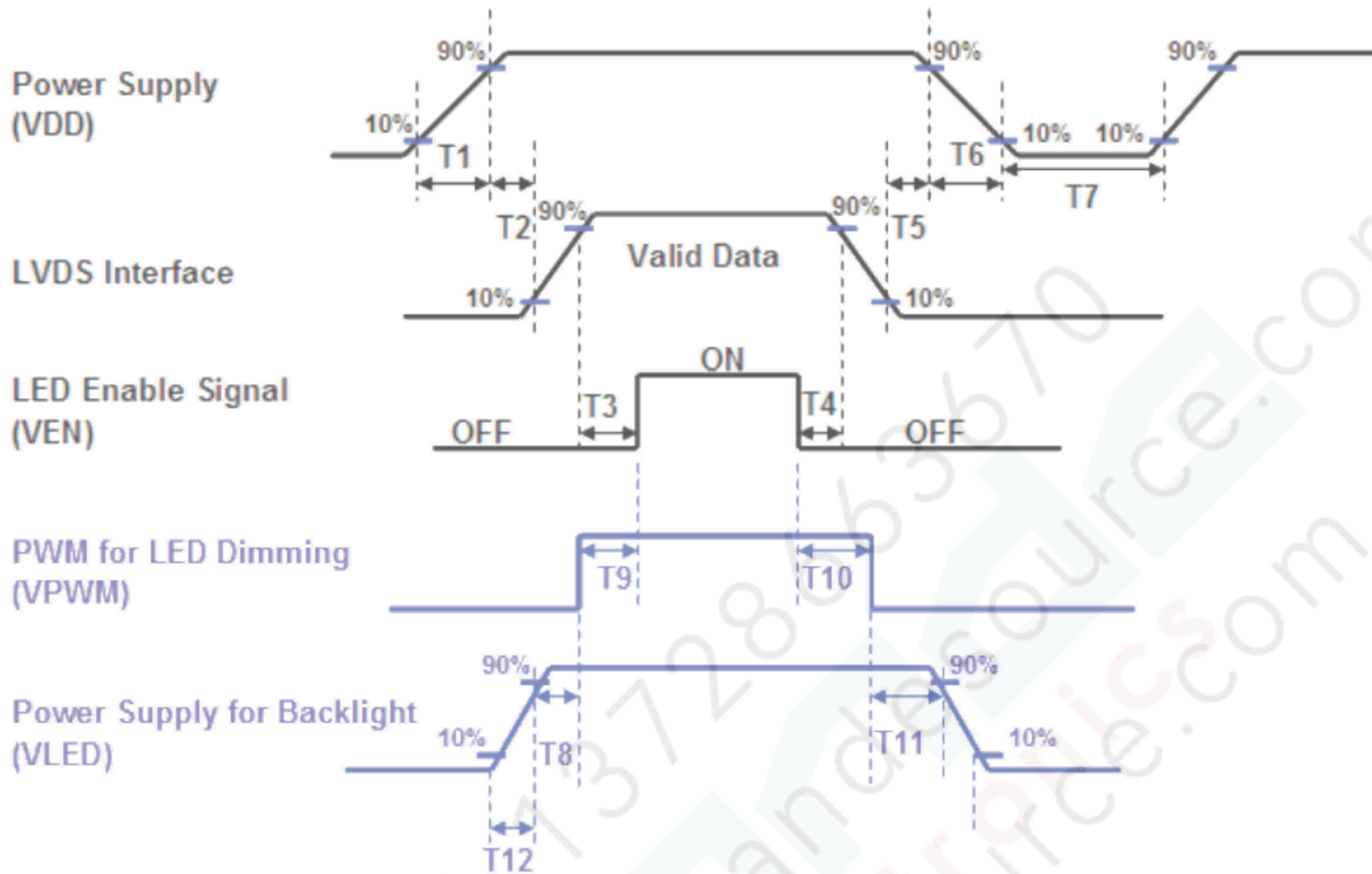
Power ON/OFF sequence timing
