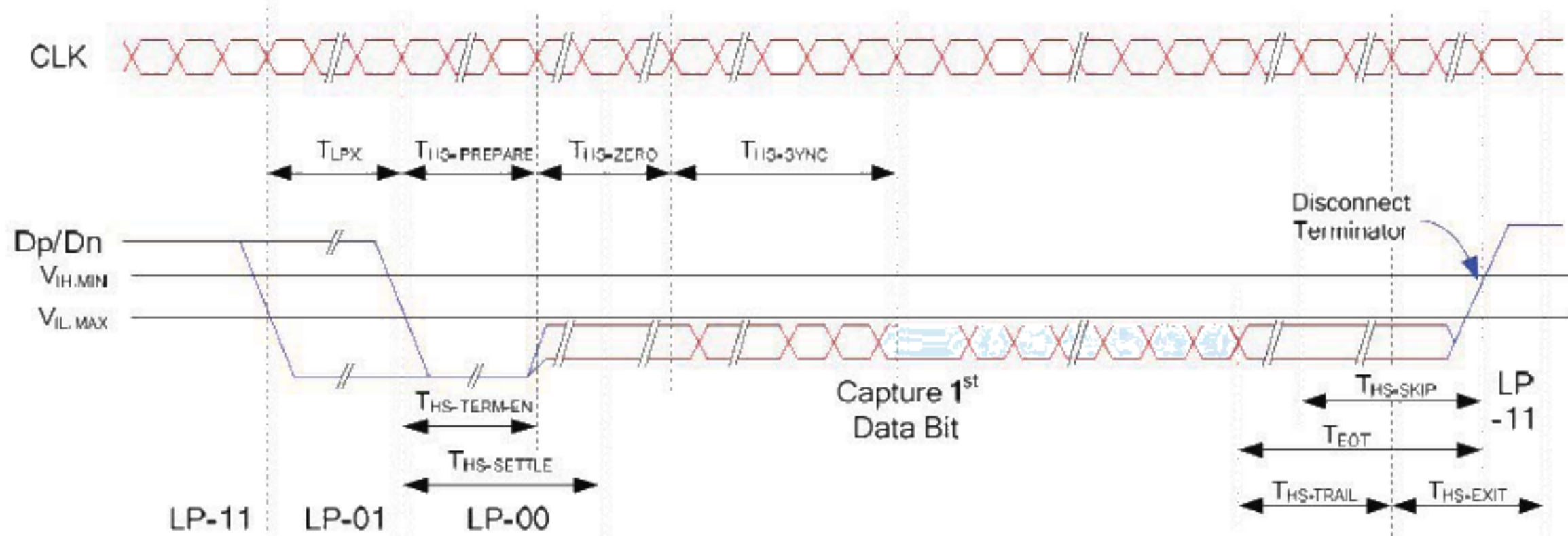
Figure : High-Speed Data Transmission in Bursts
