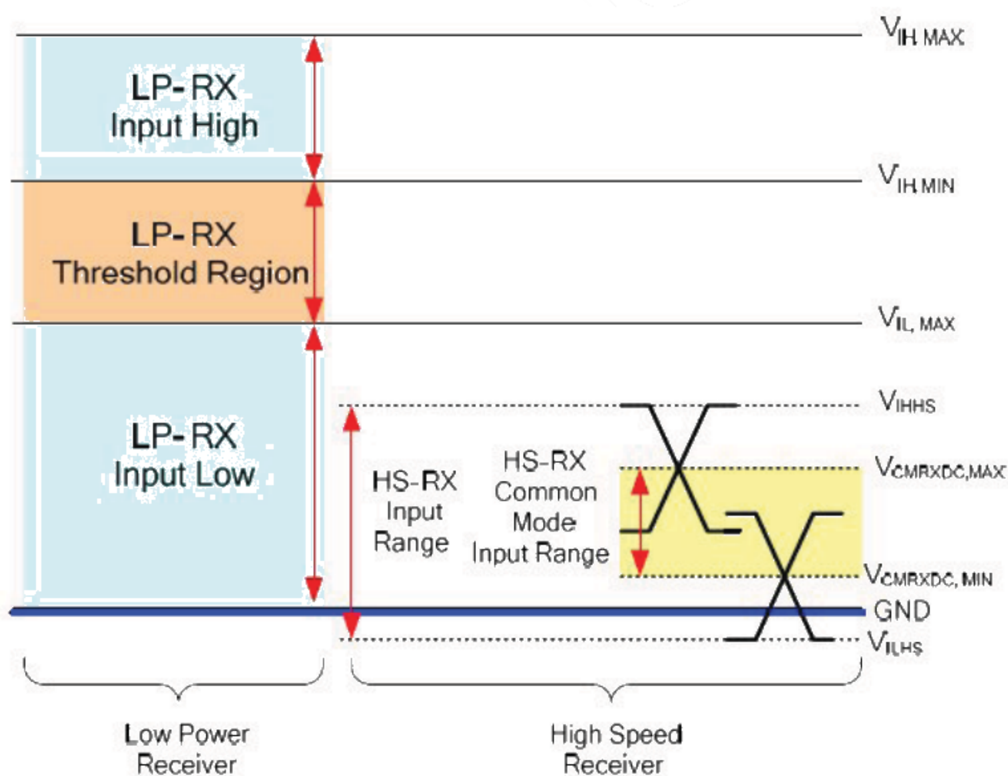
Figure: MIPI DC Diagram
