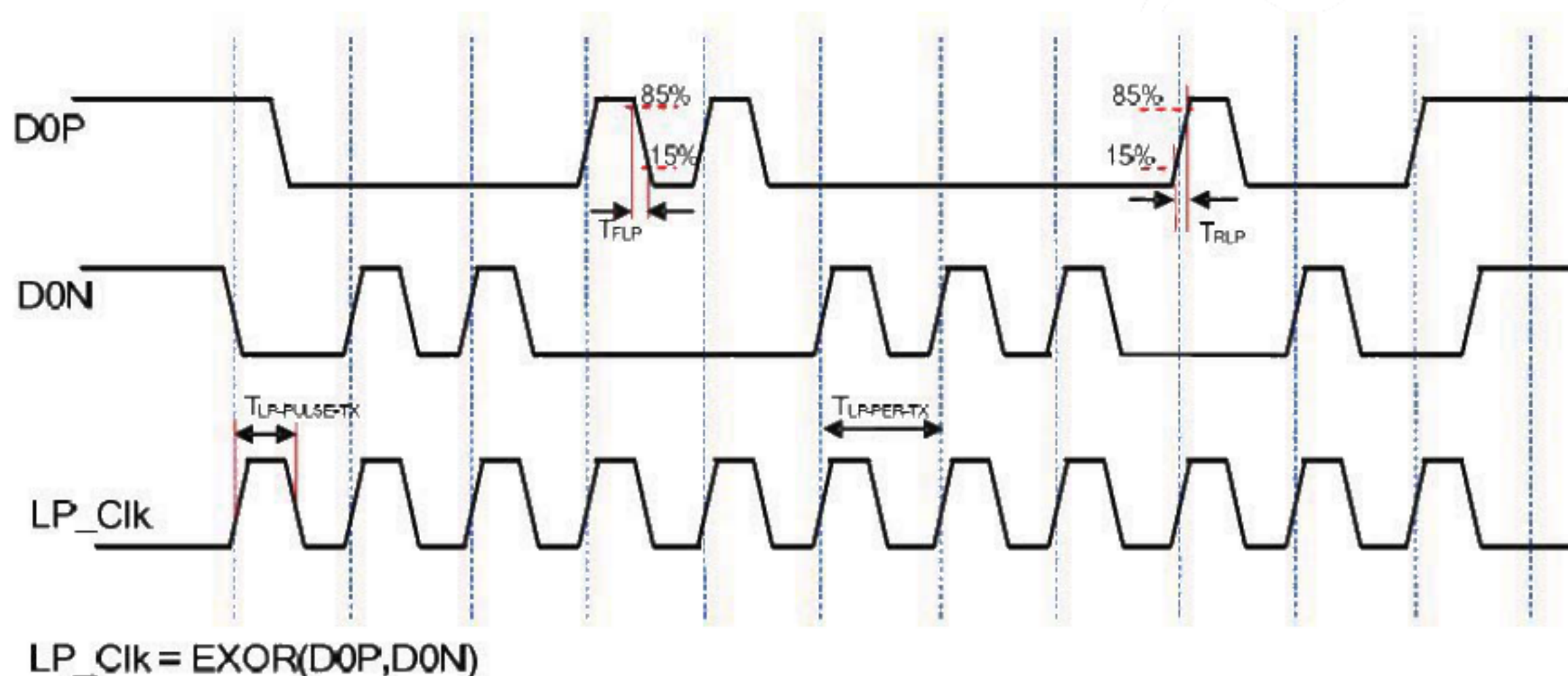
Figure: LP Transmitter Timing Definitions
