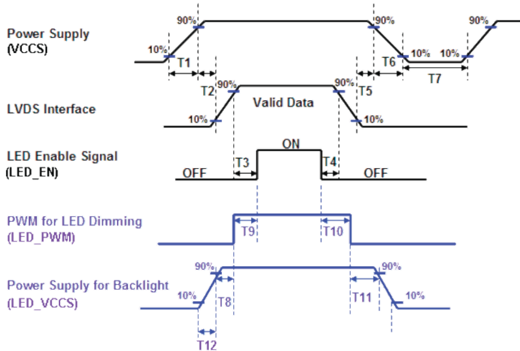
Power ON/OFF sequence timing
