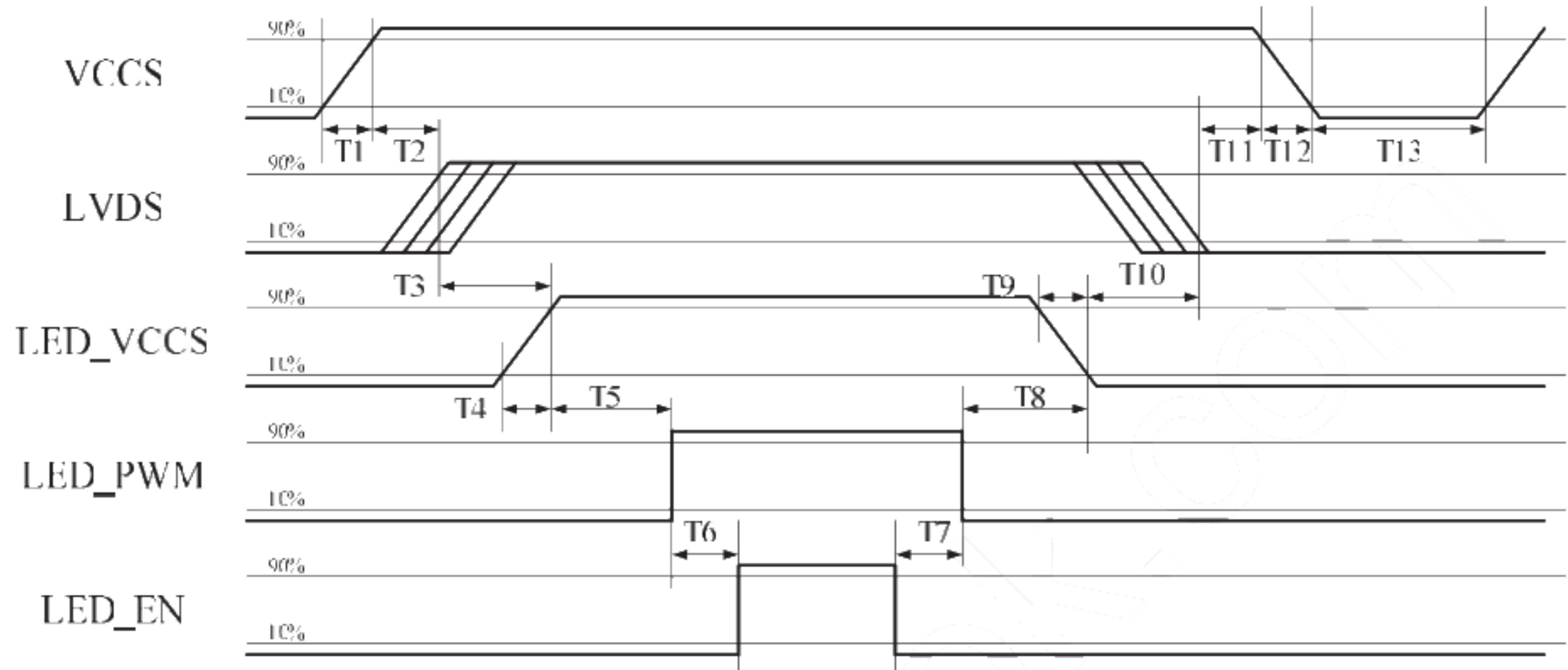
Power ON/OFF sequence timing
