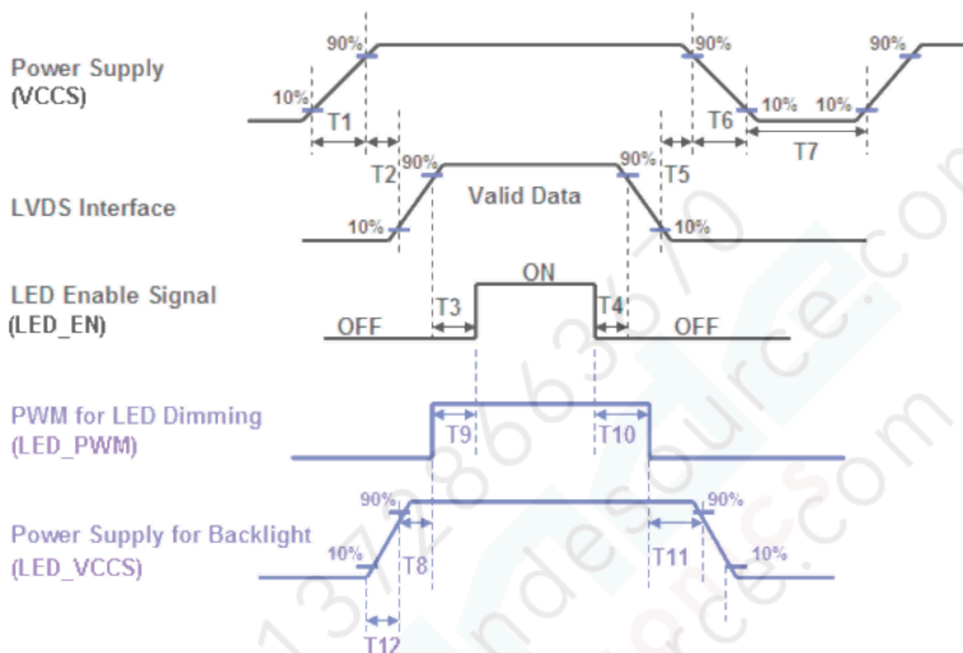
Power ON/OFF sequence timing
