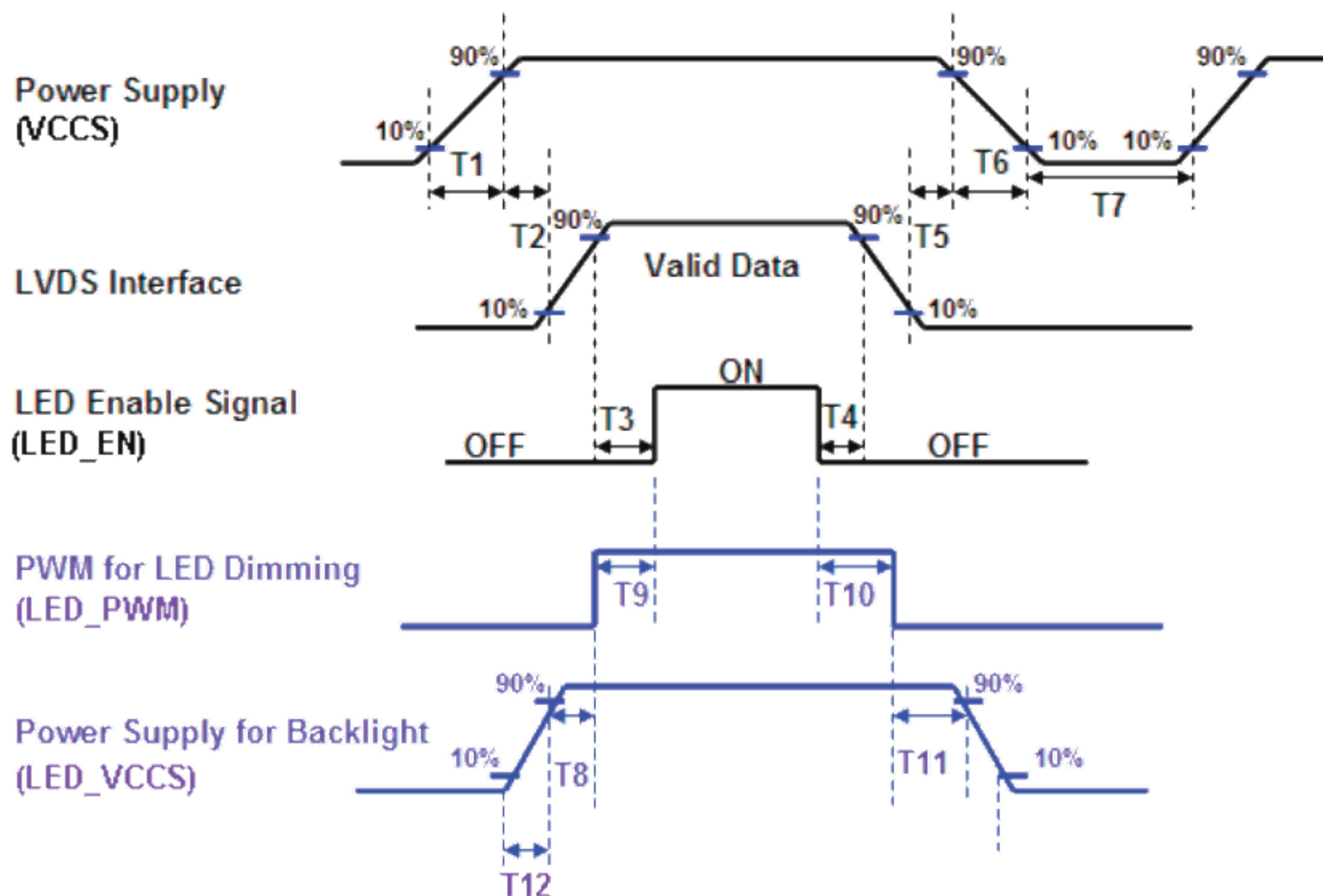
Power ON/OFF sequence timing
