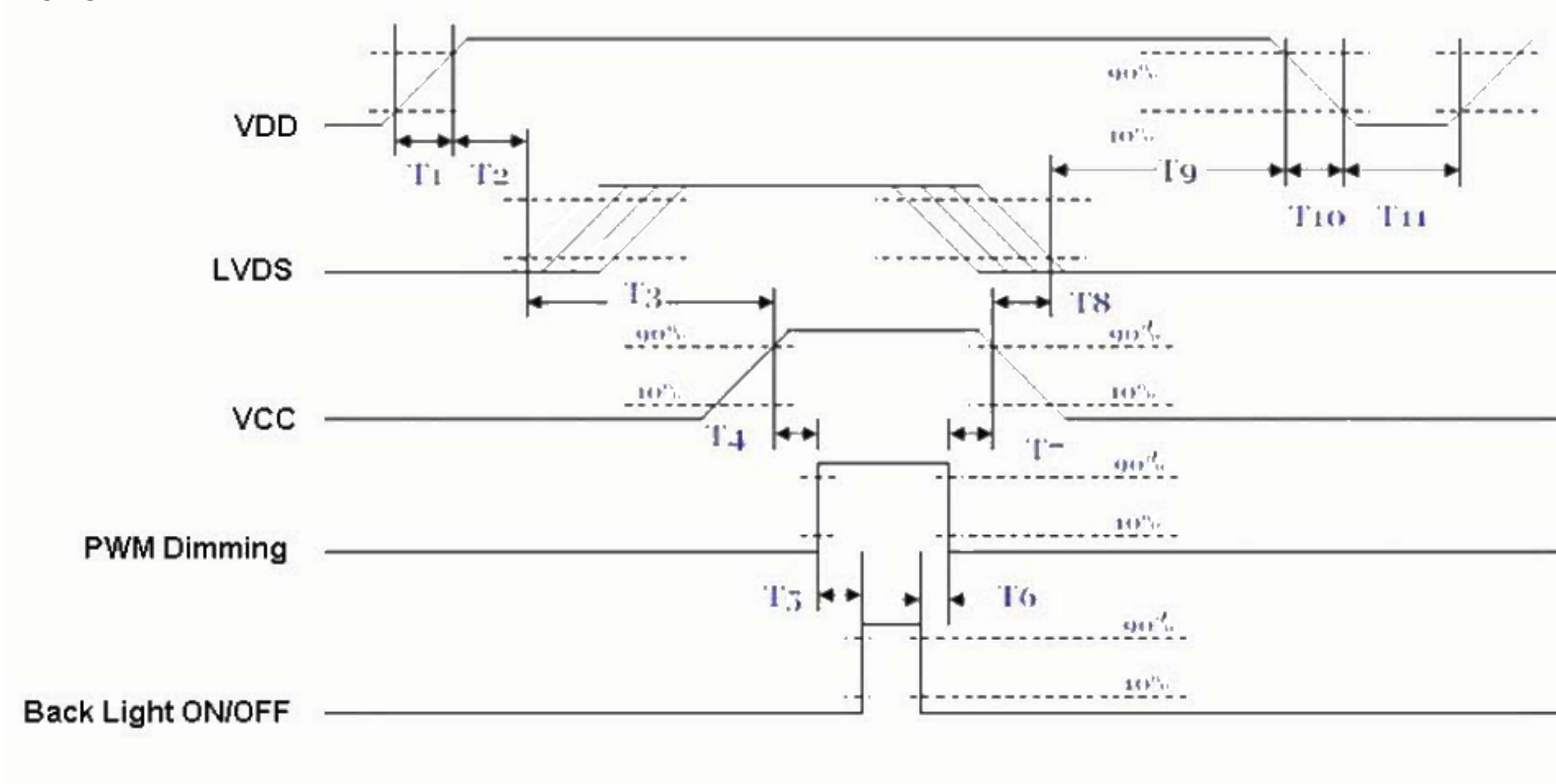
Power ON/OFF sequence timing
