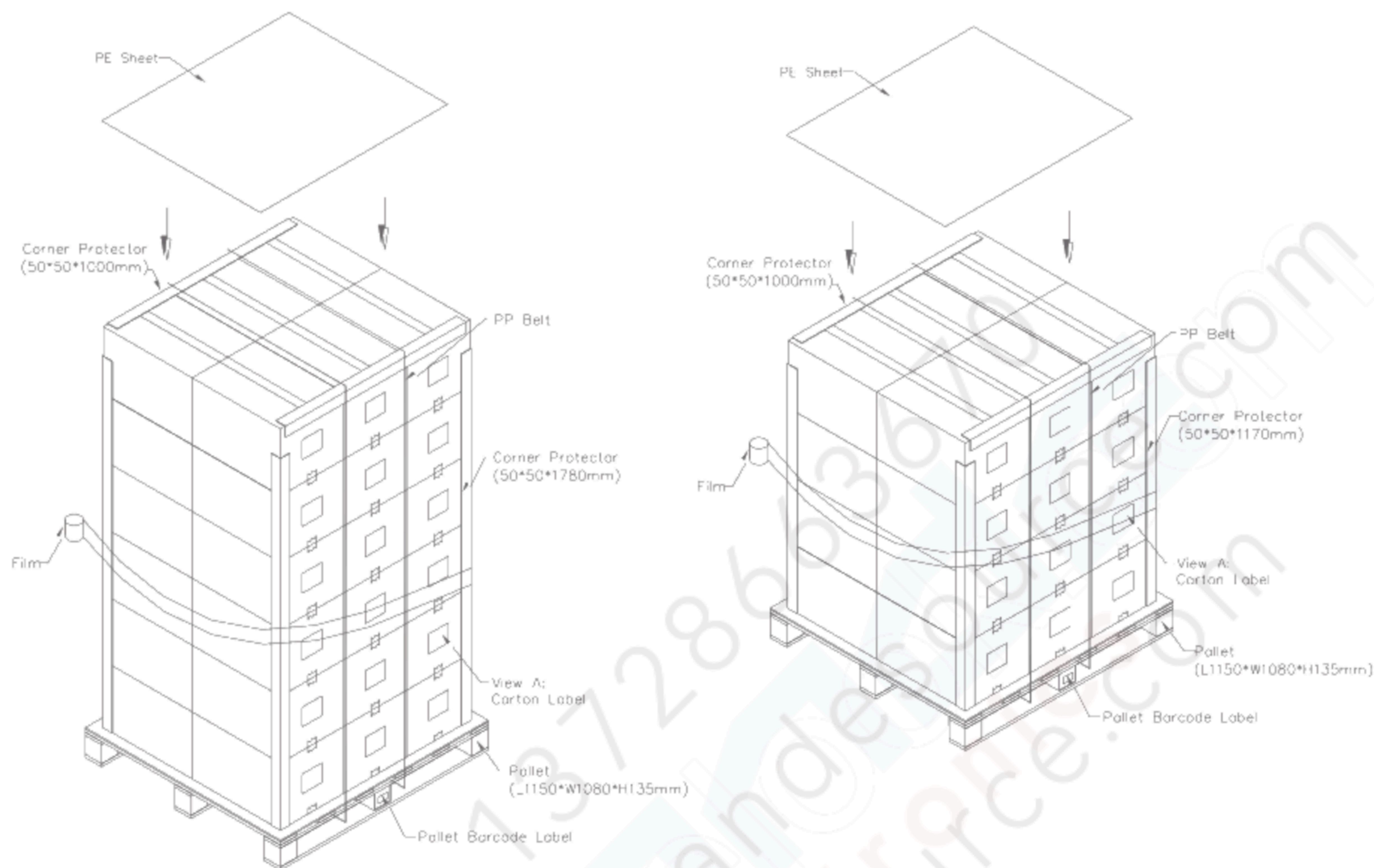
Figure. 9-2 Packing method
