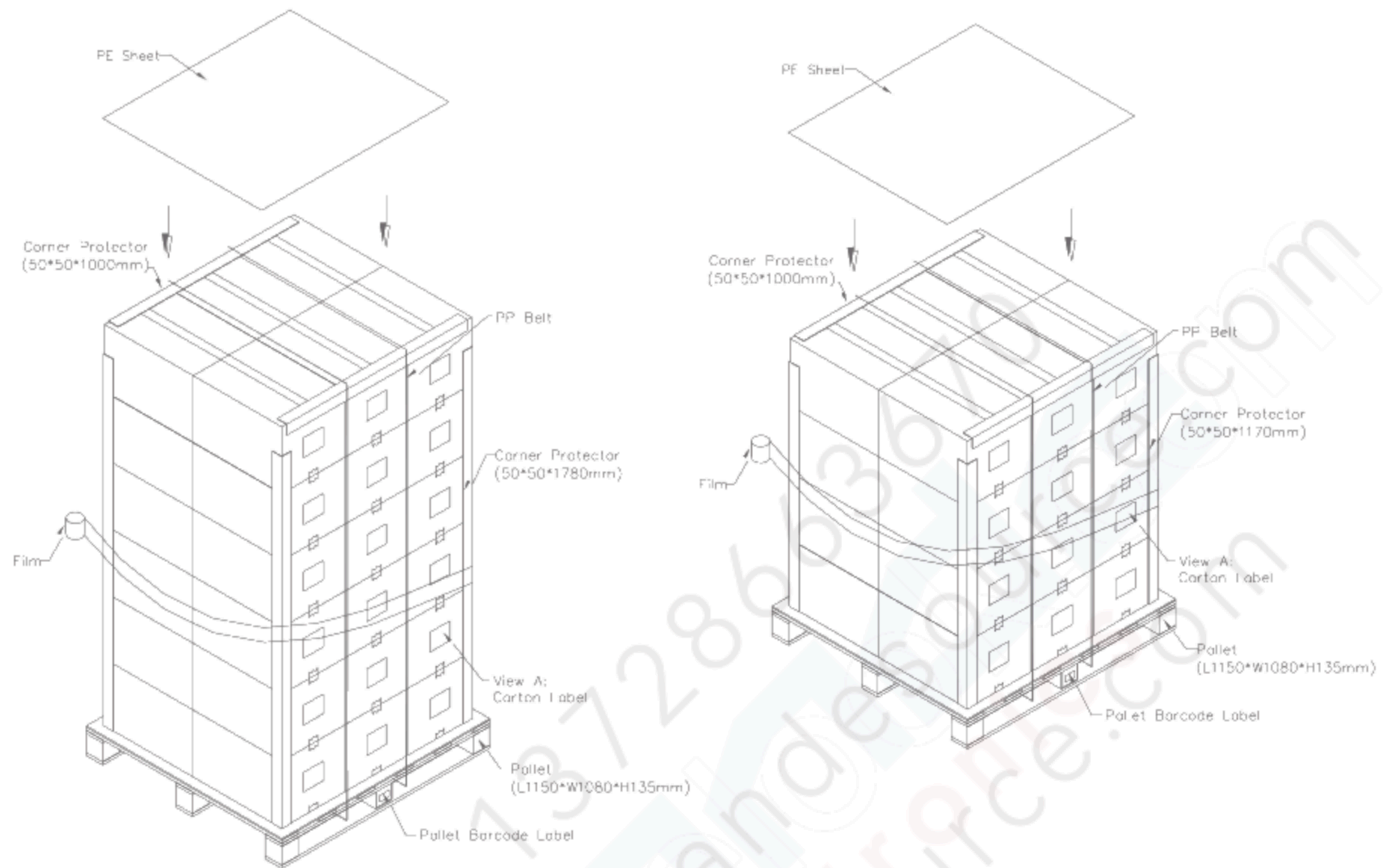
Figure. 9-2 Packing method
