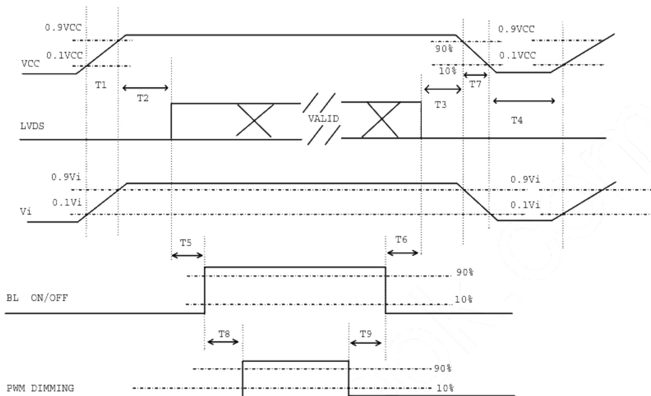
Power ON/OFF sequence
