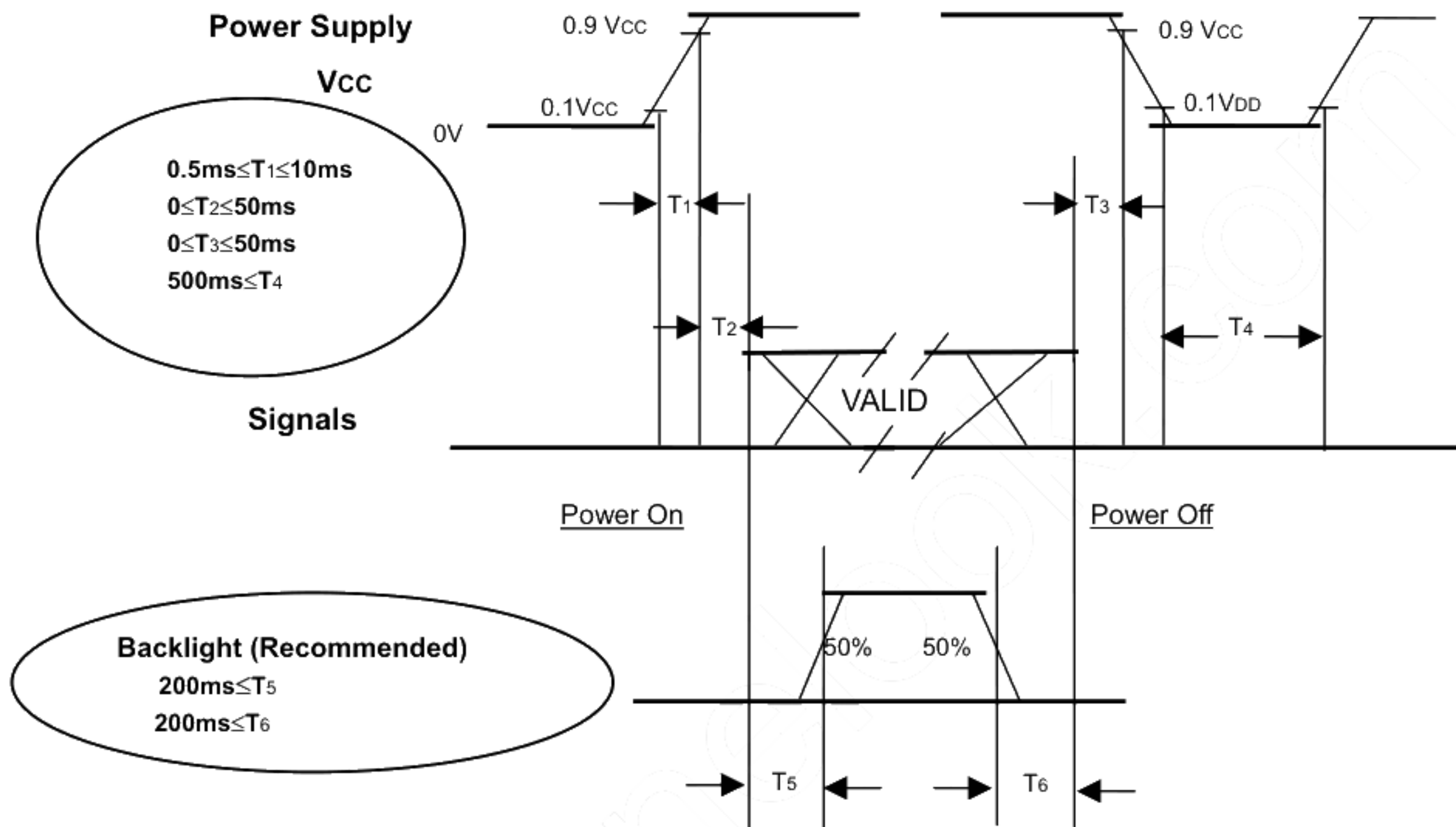
Power ON/OFF Sequence
