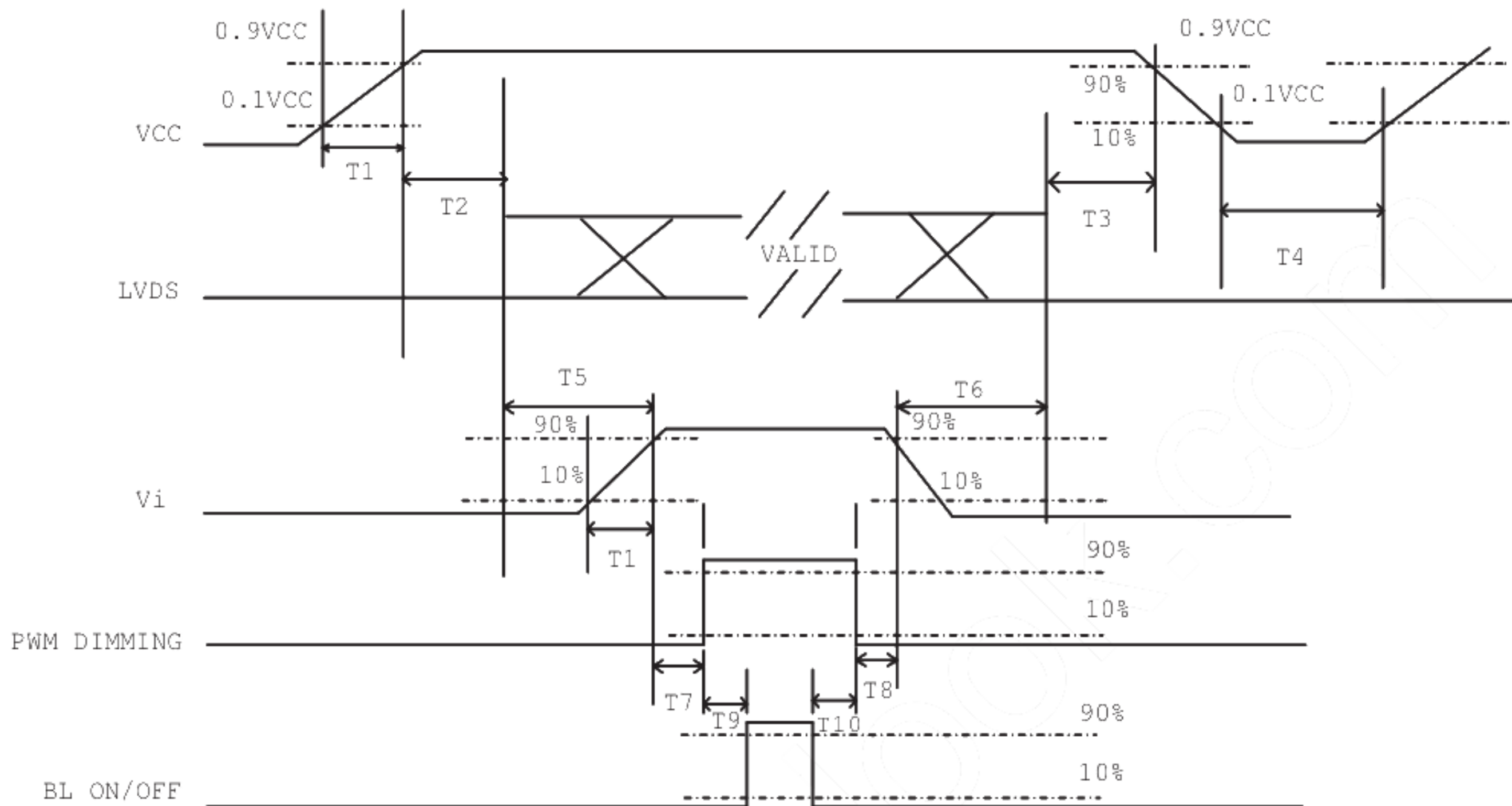
Power ON/OFF sequence
