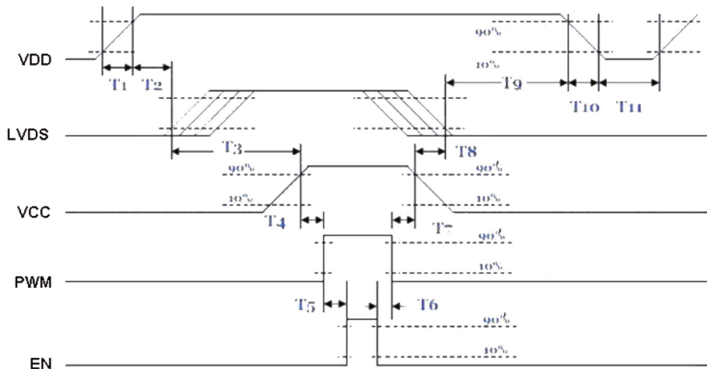
Power ON/OFF sequence timing
