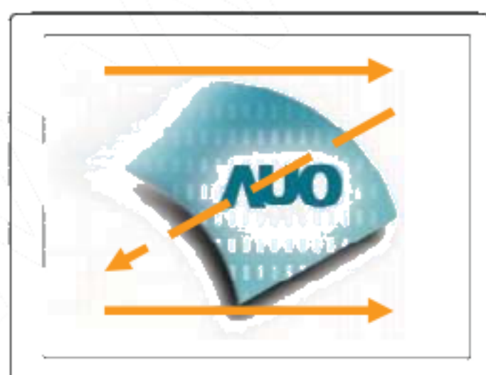
Fig. 1 Normal scan (Pin19, RSV = Low or NC)
