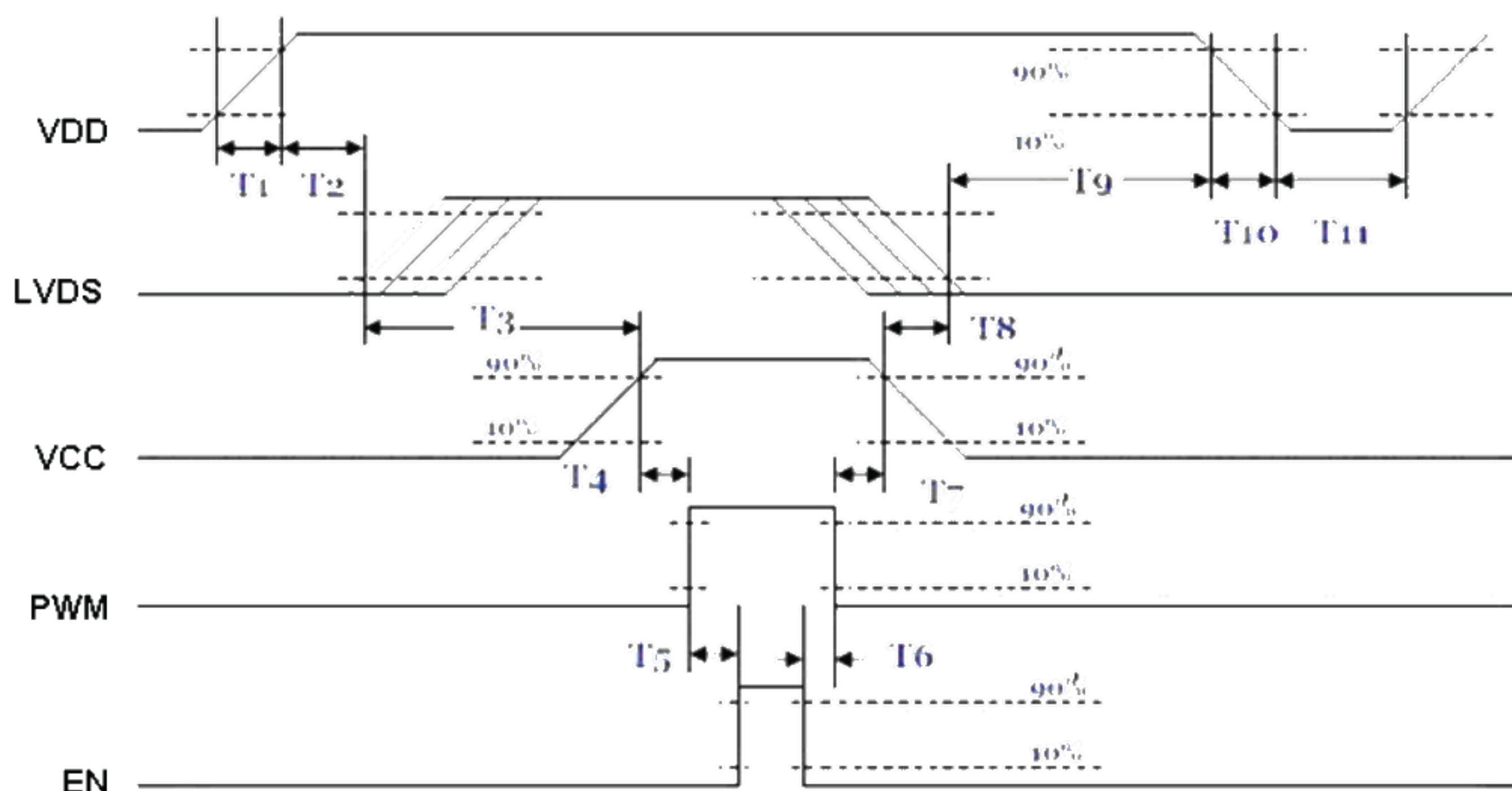
Power ON/OFF sequence timing
