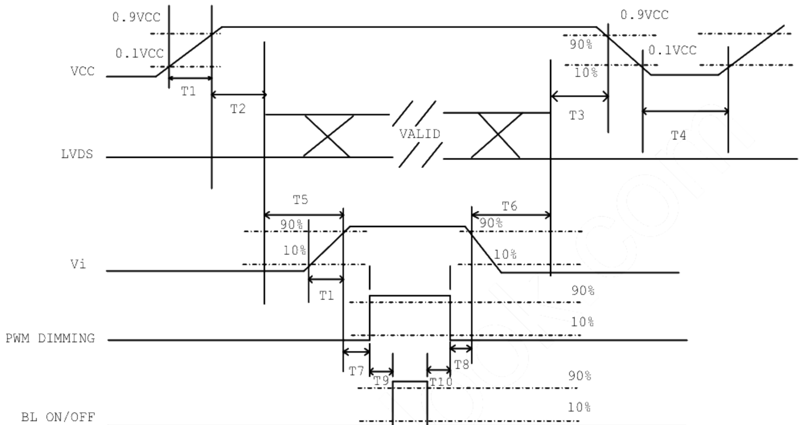
Power ON/OFF sequence
